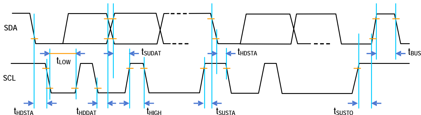
Figure 12. Timing Diagram
