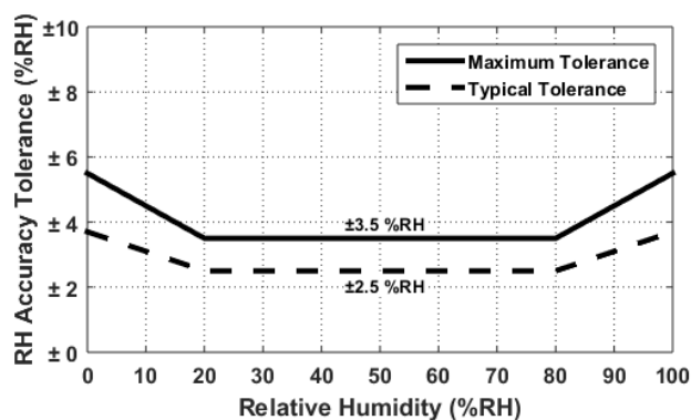
Figure 5. HS4003 RH Accuracy Tolerance at 25°C
