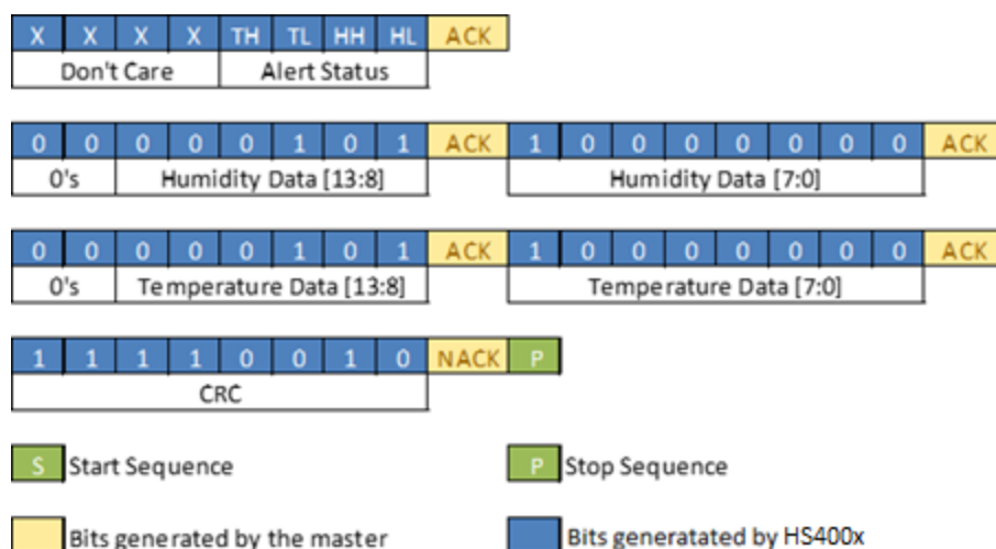
Figure 19. Data Returned from HS400x when the Alert Feature is Enabled in Periodic Measurement Mode
