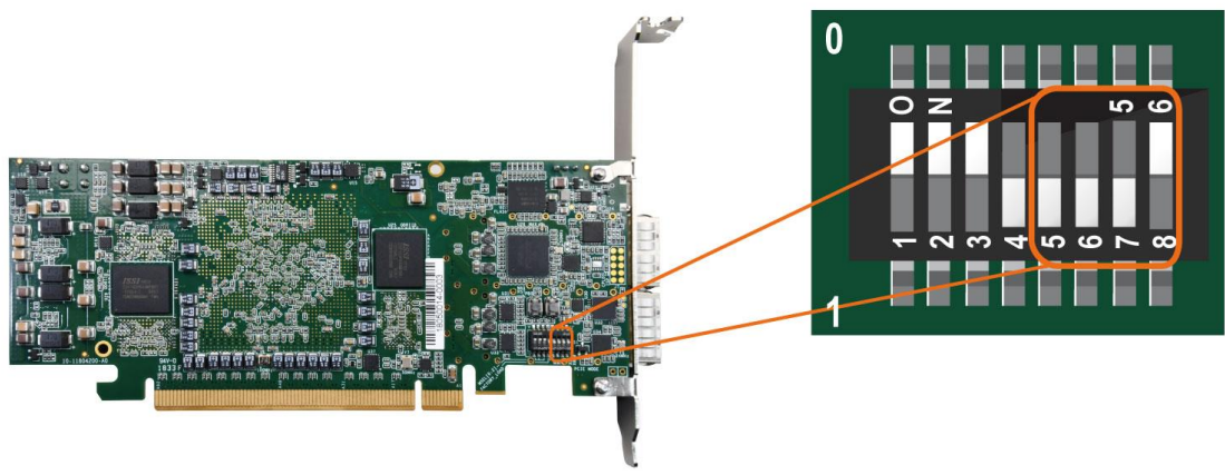
Figure 2-4 Setup PCI Express Control DIP switch
