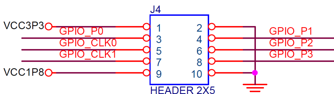
Figure 2-17 Pin-out of Timing Expansion Header
