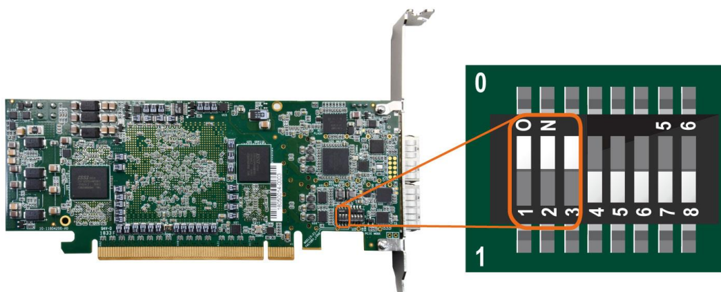
Figure 3-1 MSEL[2:0]=000
