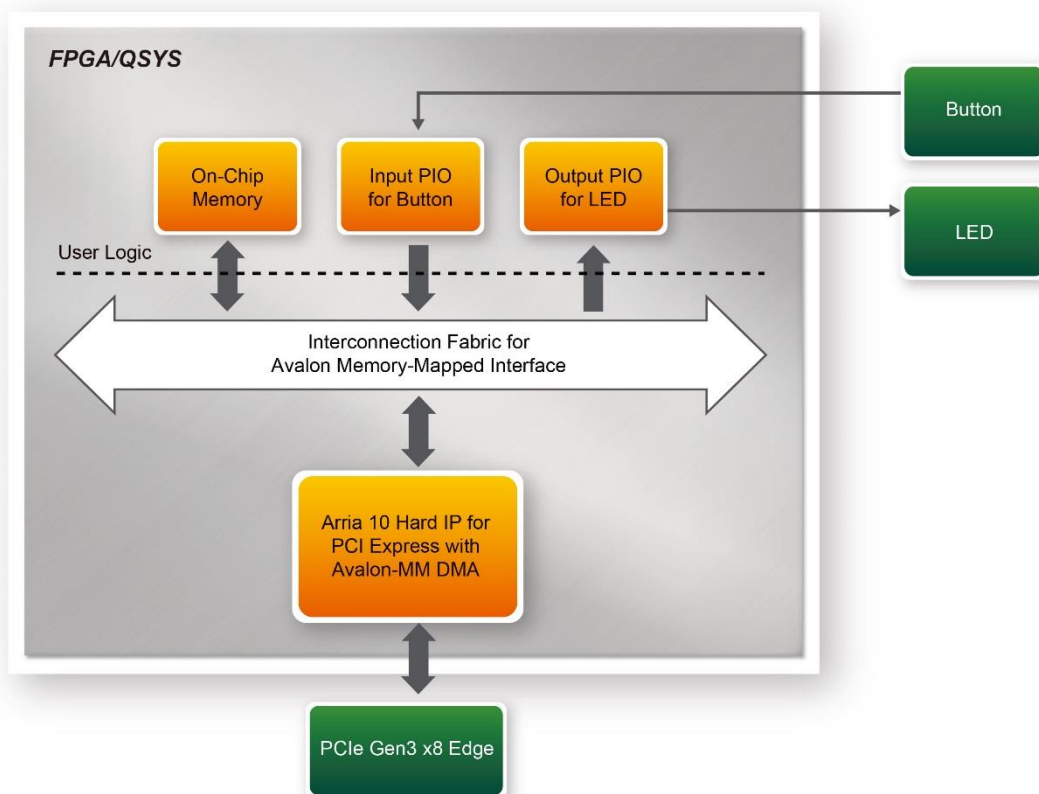
Figure 6-15 Hardware block diagram of the PCIe reference design
