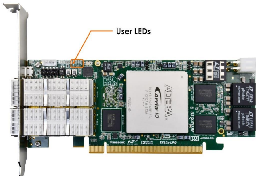
Figure 2-10 Four User LEDs
