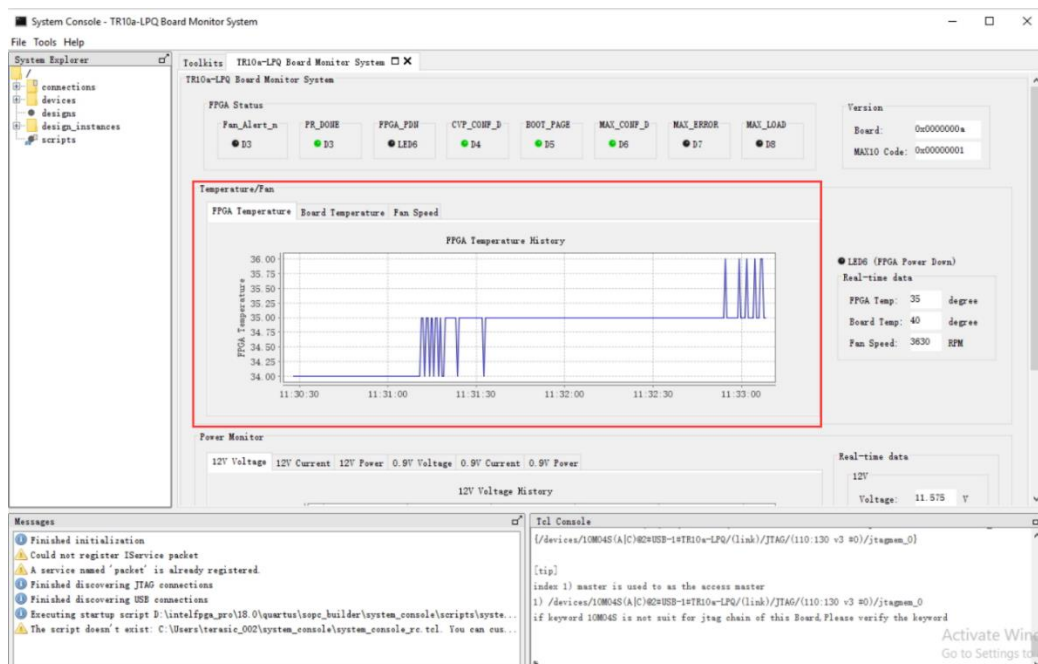
Figure 8-6 Temperature/Fan Section
