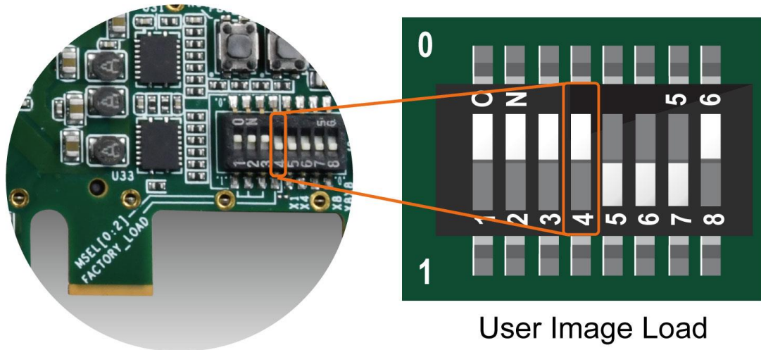
Figure 2-7 Position of DIP switch S1 for Image Select – User Image Load
