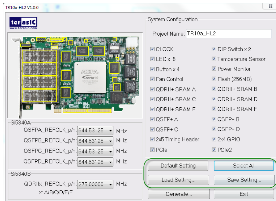
Figure 3-6 Project Settings
