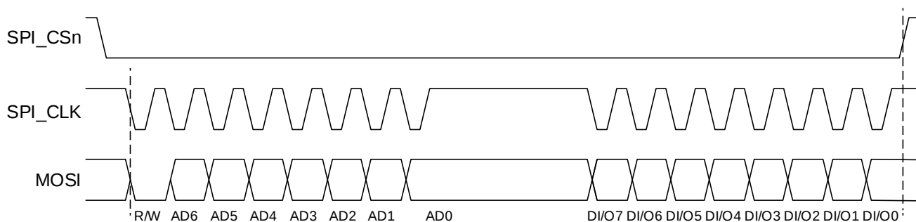
Figure 22: 3-Wire Basic SPI Read/Write Sequence (Mode 11)
