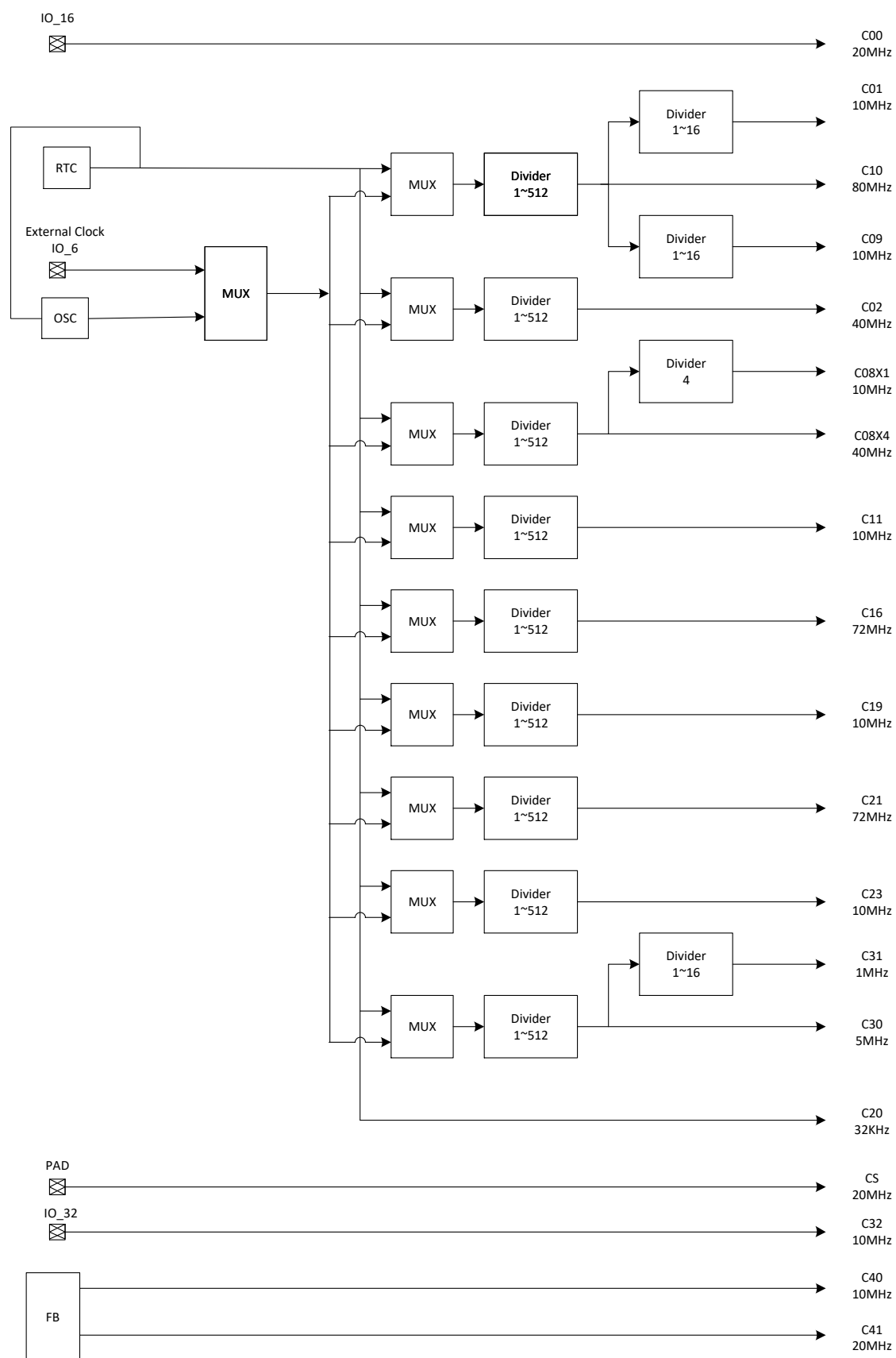
Figure 48: Clock Tree
