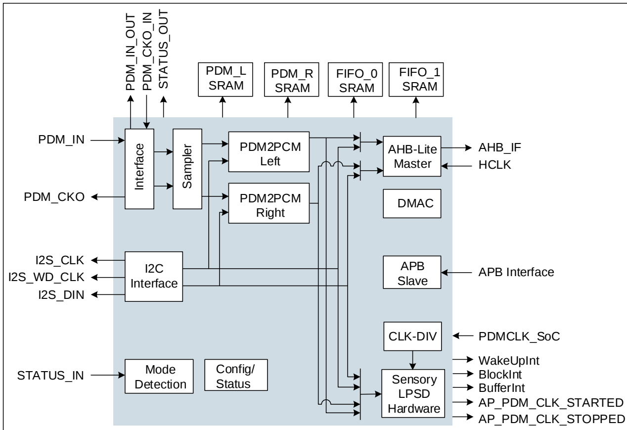
Figure 29: Voice Subsystem Block Diagram
