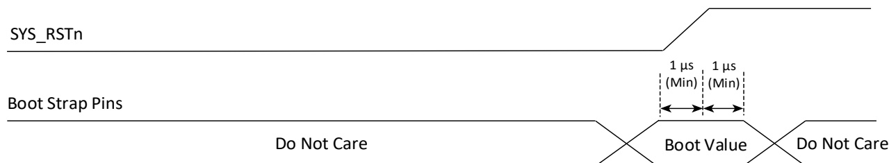
Figure 49: Bootstrap Timing
