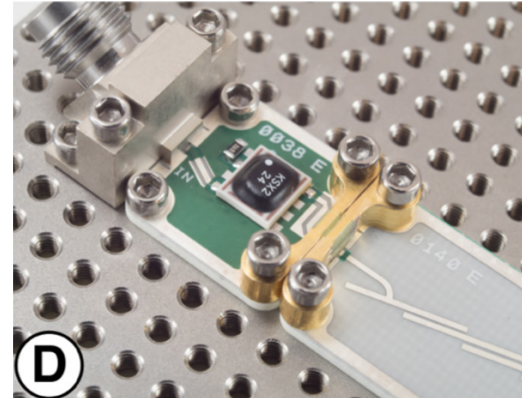
D Each side of the GSG jumper is secured by an anchor.
