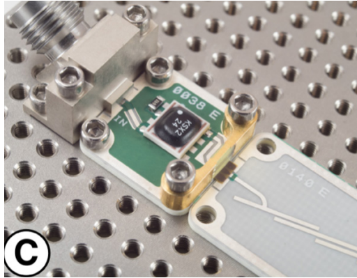
C An X-MWanchor secures a jumper across the 5 mil air gap.
