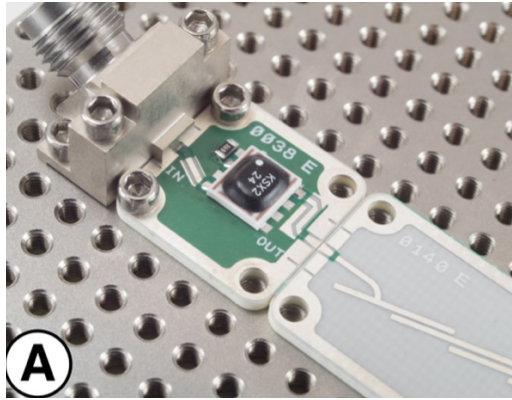
A X-MWblocks on a prototyping plate.
