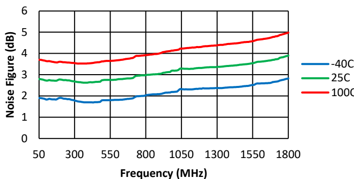
Noise Figure vs Frequency
