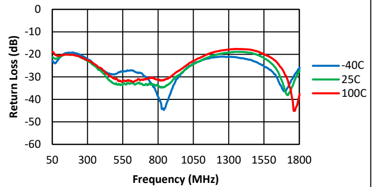
Output Return Loss vs Frequency
