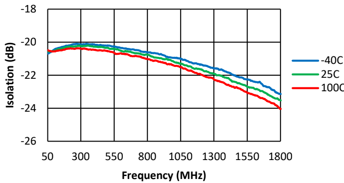
Reverse Isolation vs Frequency
