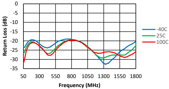
Input Return Loss vs Frequency
