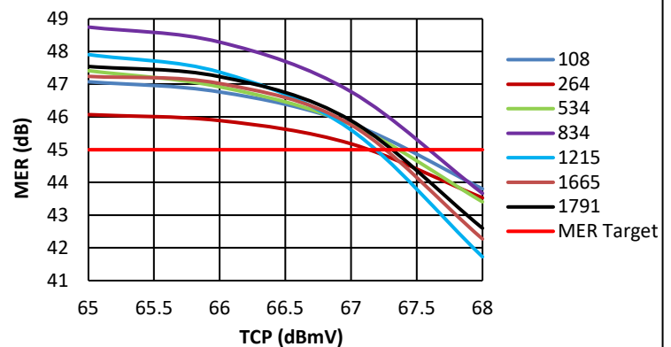
QPL1822 MER vs TCP at 8V
