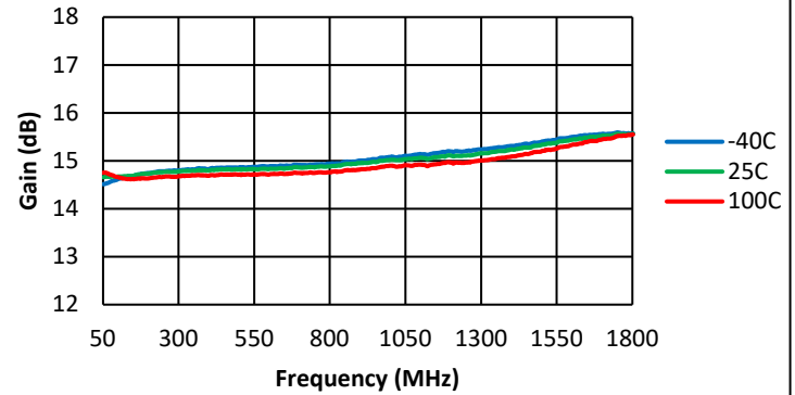
Gain vs Frequency
