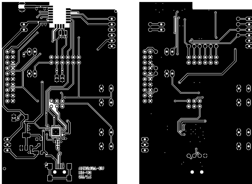
Figure 18: Top & bottom Layer
