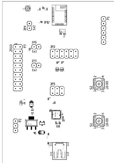
Figure 17: Assembly diagram
