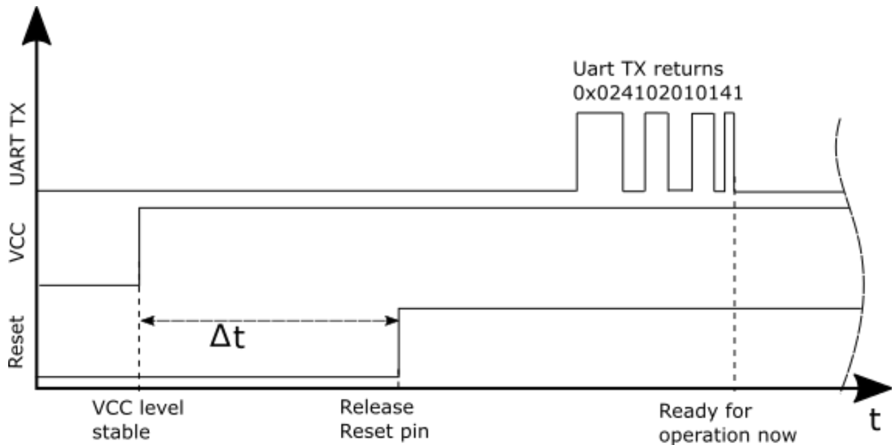
Figure 6: Power up
