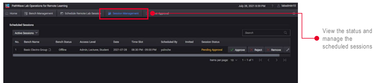
Figure 5. Administrator to view, approve or reject the scheduled lab sessions
