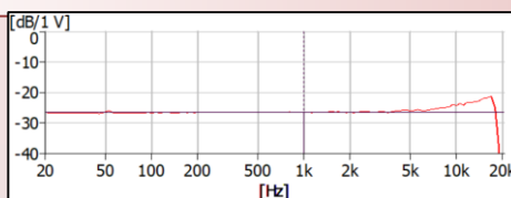
Frequency Response
