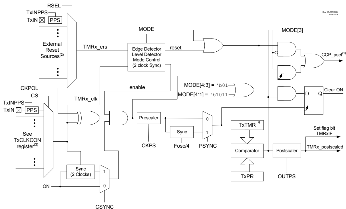
Figure 29-1. Timer2 with Hardware Limit Timer (HLT) Block Diagram
