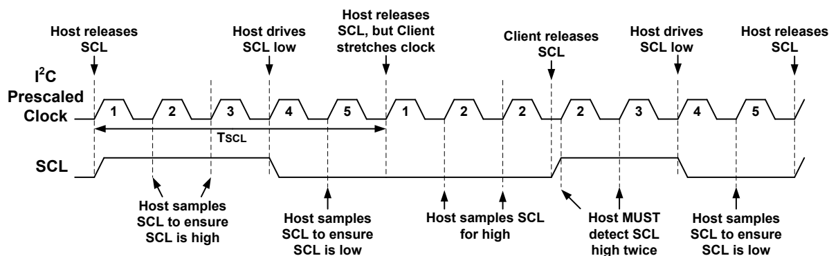
Figure 39-30. SCL Timing (FME = 0, up to f_{SCL} = 100 kHz)
