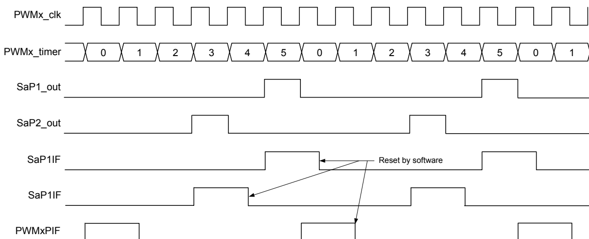
Figure 33-10. Pulsed Compare Timing Diagram
