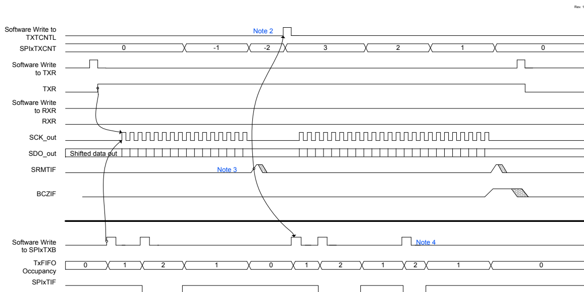
Figure 38-4. SPI Host Operation - Command+Write Data, TXR = 1, RXR = 0
