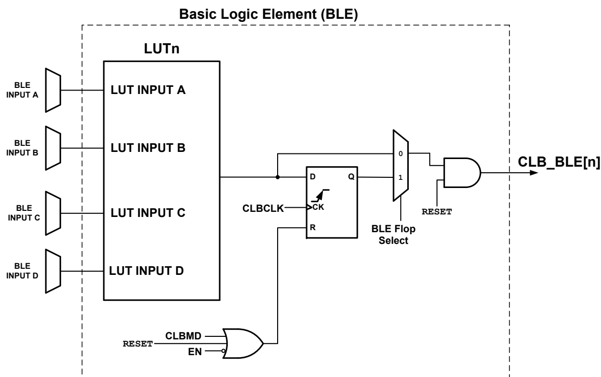
Figure 25-1. Basic Logic Element (BLE) Simplified Block Diagram
