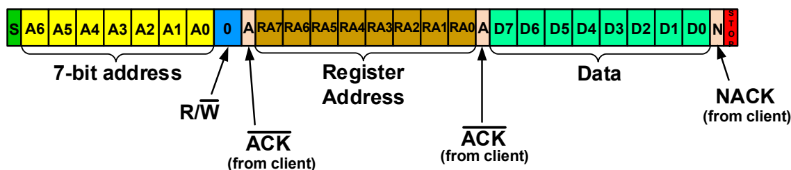
Figure 39-28. 10-Bit Host Write Diagram
