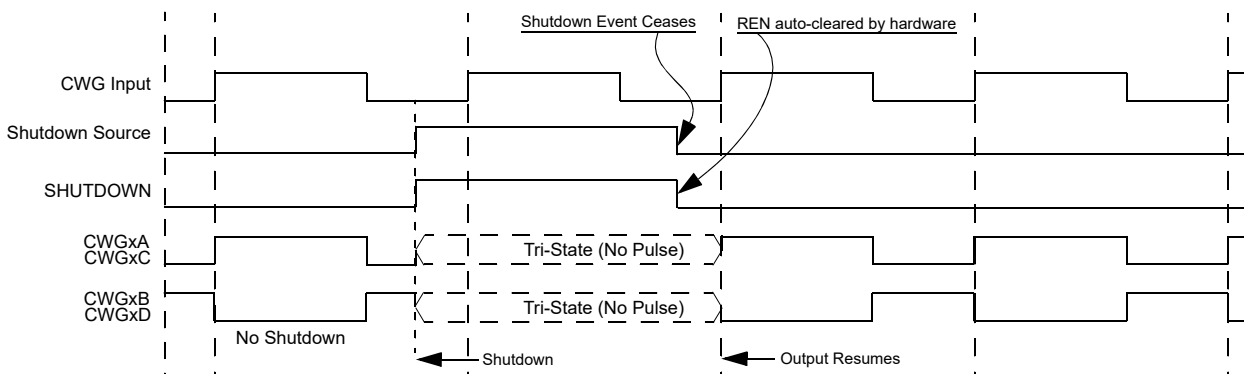
Figure 34-16. Shutdown Functionality, Auto-Restart Enabled (REN = 1, LSAC = 'b01, LSB0 = 'b01)
