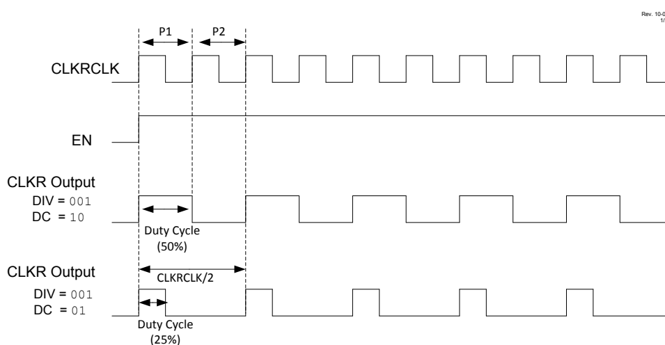
Figure 26-2. Clock Reference Timing
