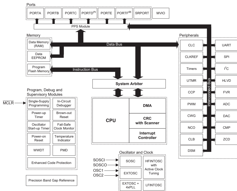
Figure 1. PIC18F26/46/56Q35 Block Diagram
