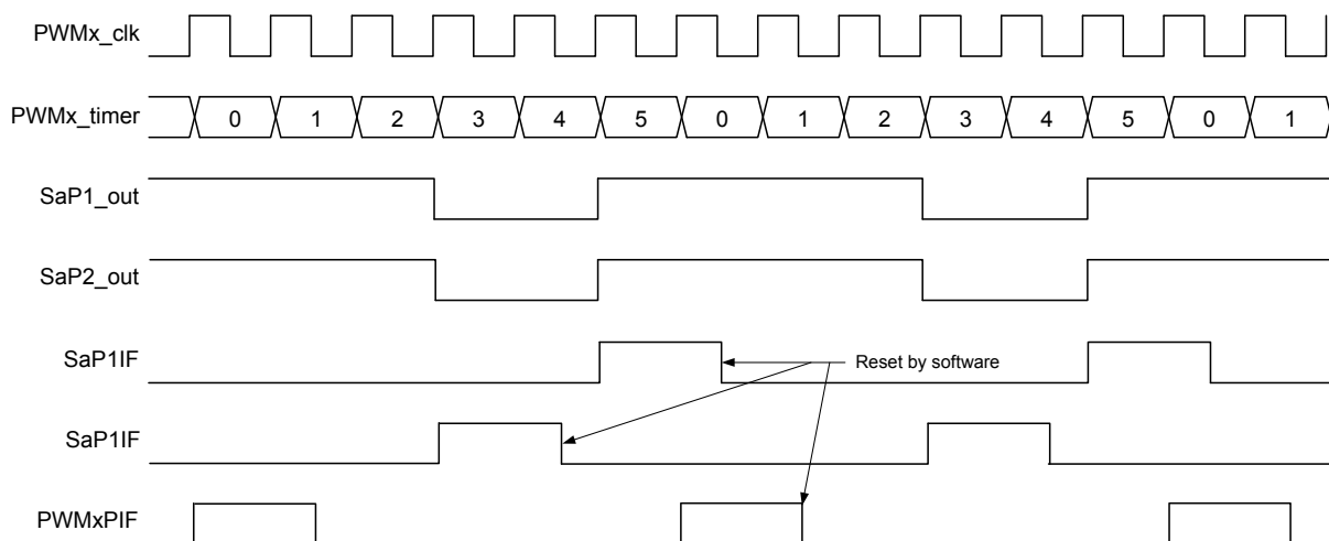
Figure 33-8. Variable Alignment Timing Diagram
