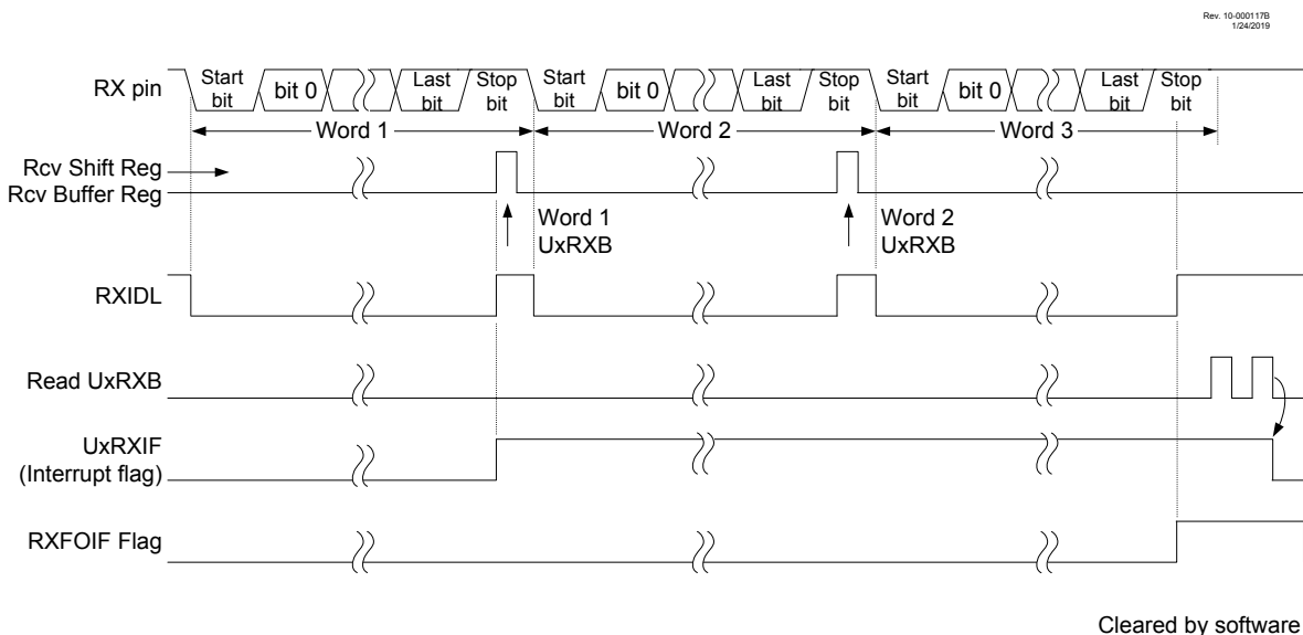
Figure 37-5. UART Asynchronous Reception
