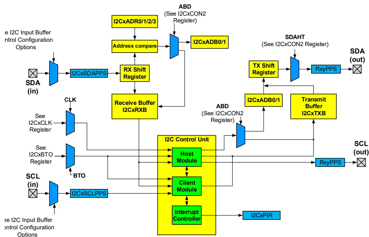
Figure 39-1. I 2 C Block Diagram
