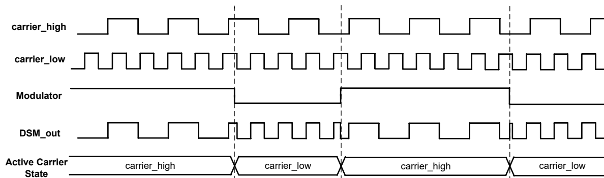
Figure 36-3. No Synchronization (MDCHSYNC = 0, MDCLSYNC = 0)
