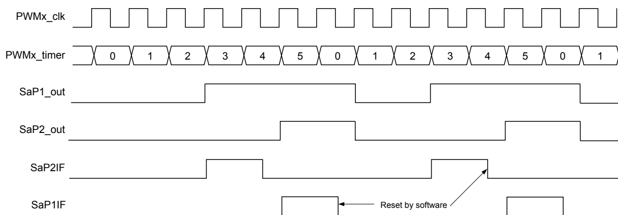
Figure 33-4. Right-Aligned Timing Diagram
