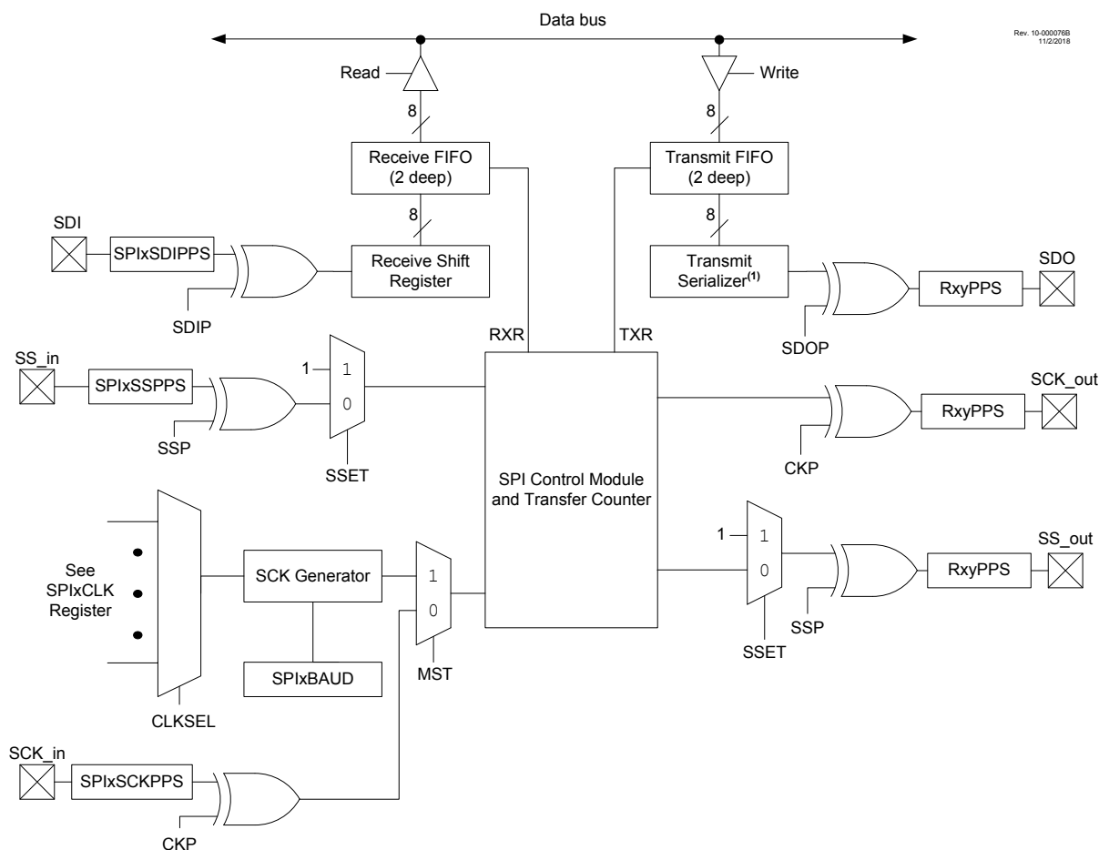
Figure 38-1. SPI Module Simplified Block Diagram
