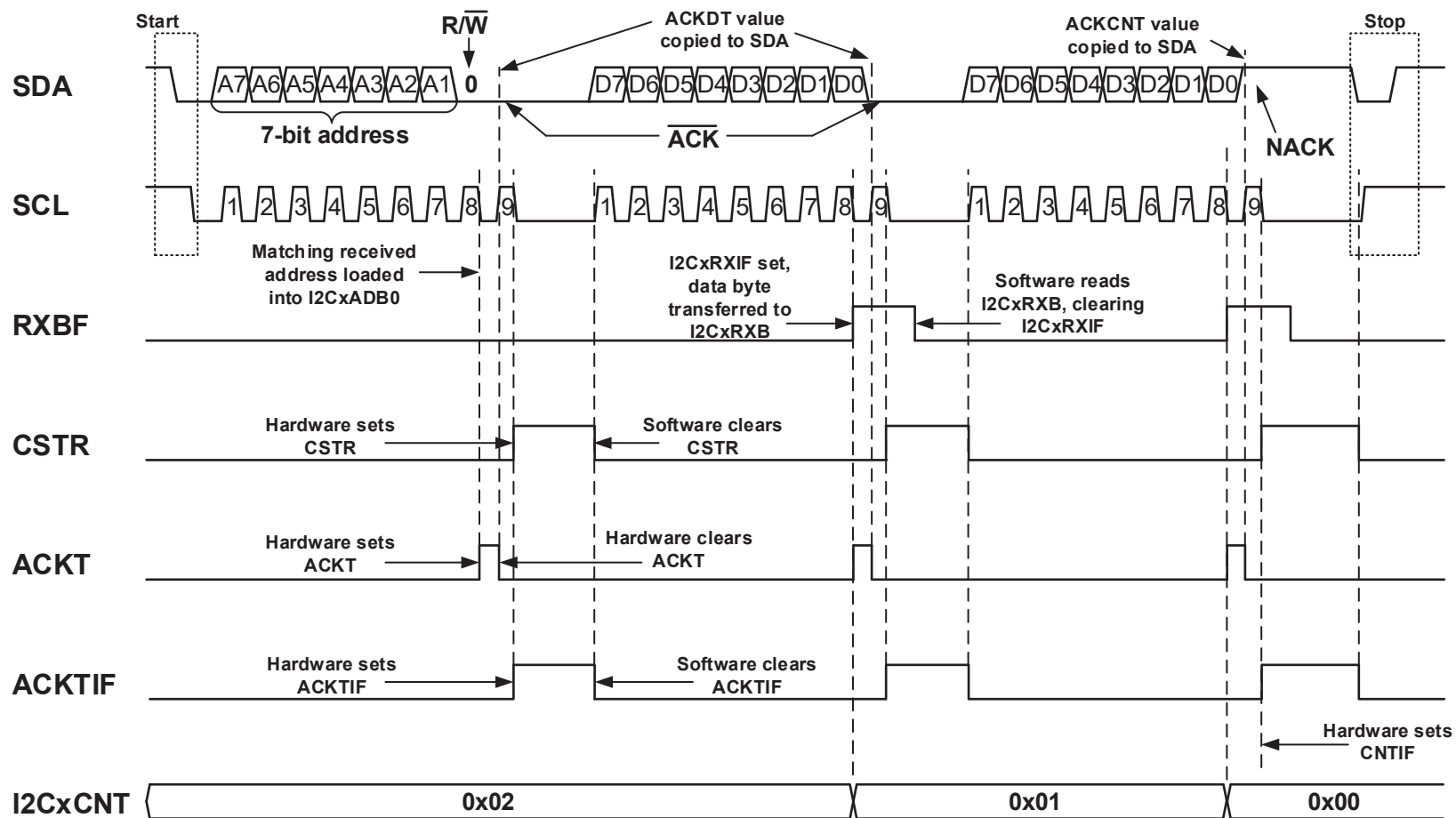
Figure 39-18. 7-Bit Client Mode Reception (ACKTIE = 1)
