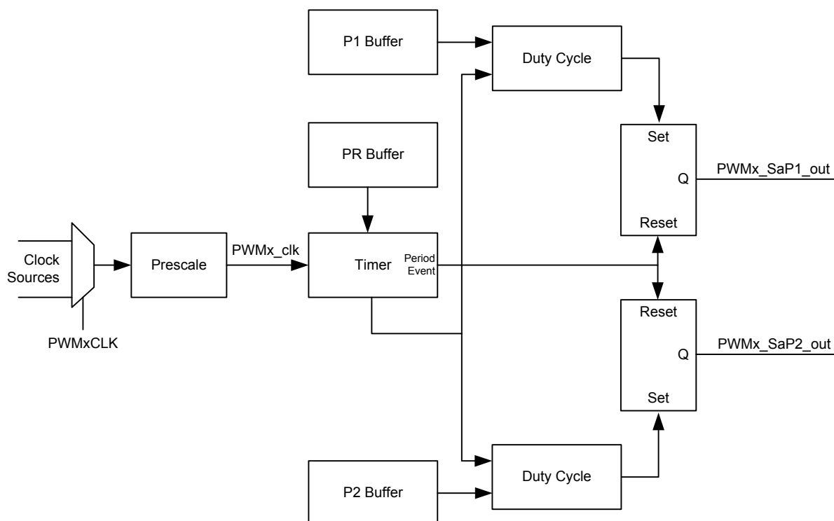
Figure 33-3. Right-Aligned Block Diagram
