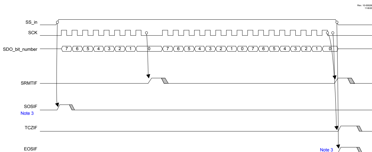
Figure 38-14. Transfer And Client Select Interrupt Timing
