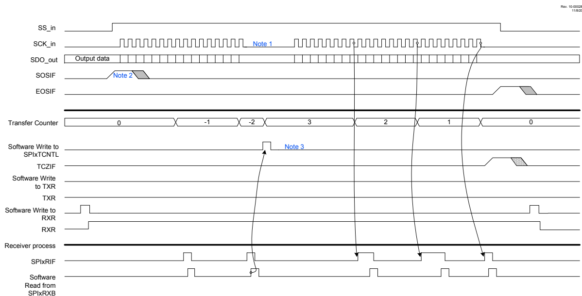
Figure 38-11. SPI Client Mode Operation – Interrupt-Driven, Host Writes 2+3 Bytes
