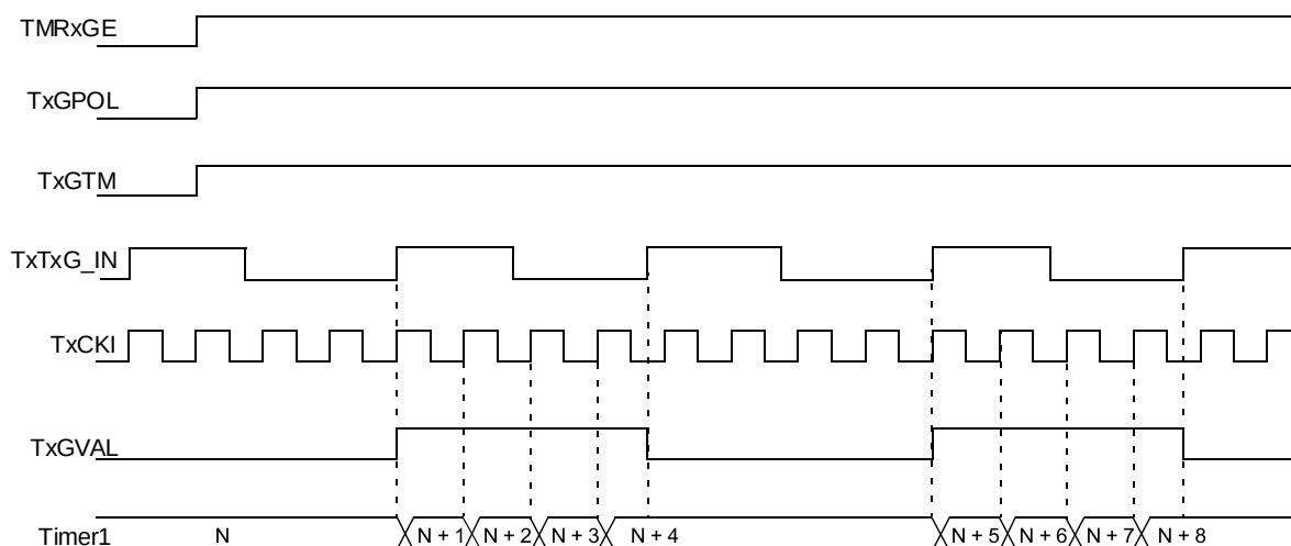
Figure 28-5. Timer1 Gate Toggle Mode
