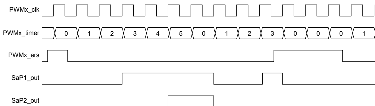
Figure 33-15. Right Aligned Mode with ERSNOW = 1
