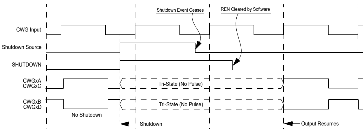
Figure 34-15. Shutdown Functionality, Auto-Restart Disabled (REN = 0, LSAC = 'b01, LSB0 = 'b01)
