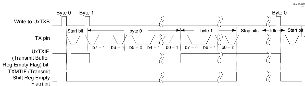
Figure 37-9. Manchester Timing
