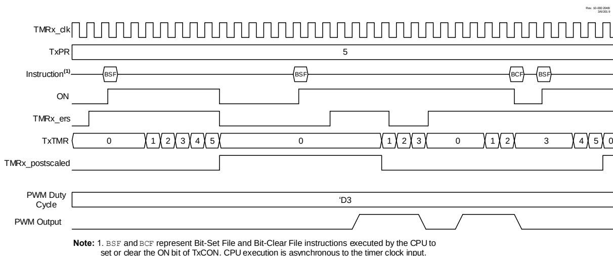
Figure 29-12. Level Triggered Hardware Limit One Shot Mode Timing Diagram (MODE = 'b10110)
