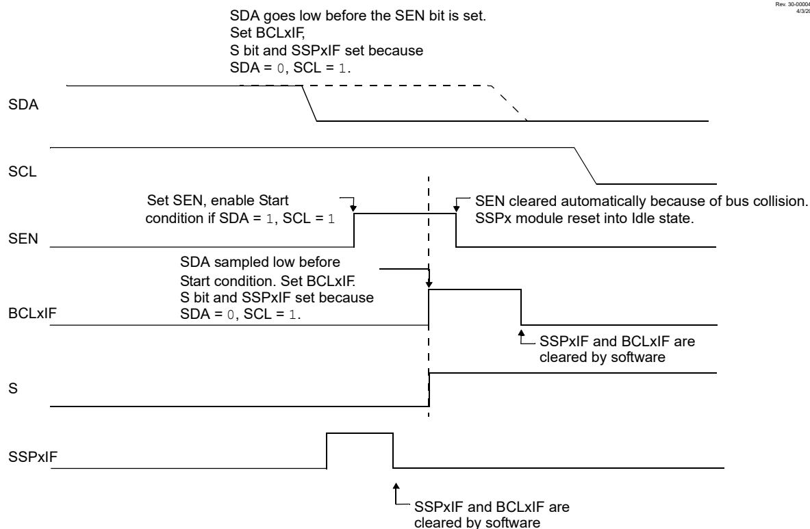
Figure 28-34. Bus Collision During Start Condition (SDA Only)
