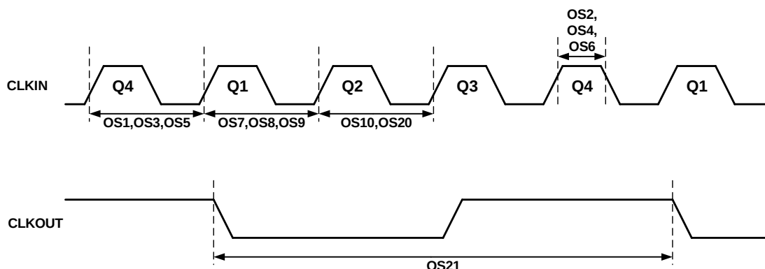
Figure 40-4. Clock Timing
