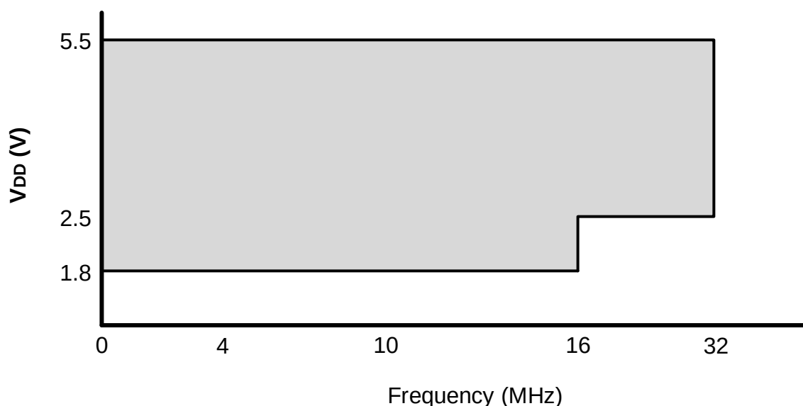
Figure 40-1. Voltage Frequency Graph, -40^{\circ}\text{C} \leq T_A \leq +125^{\circ}\text{C}
