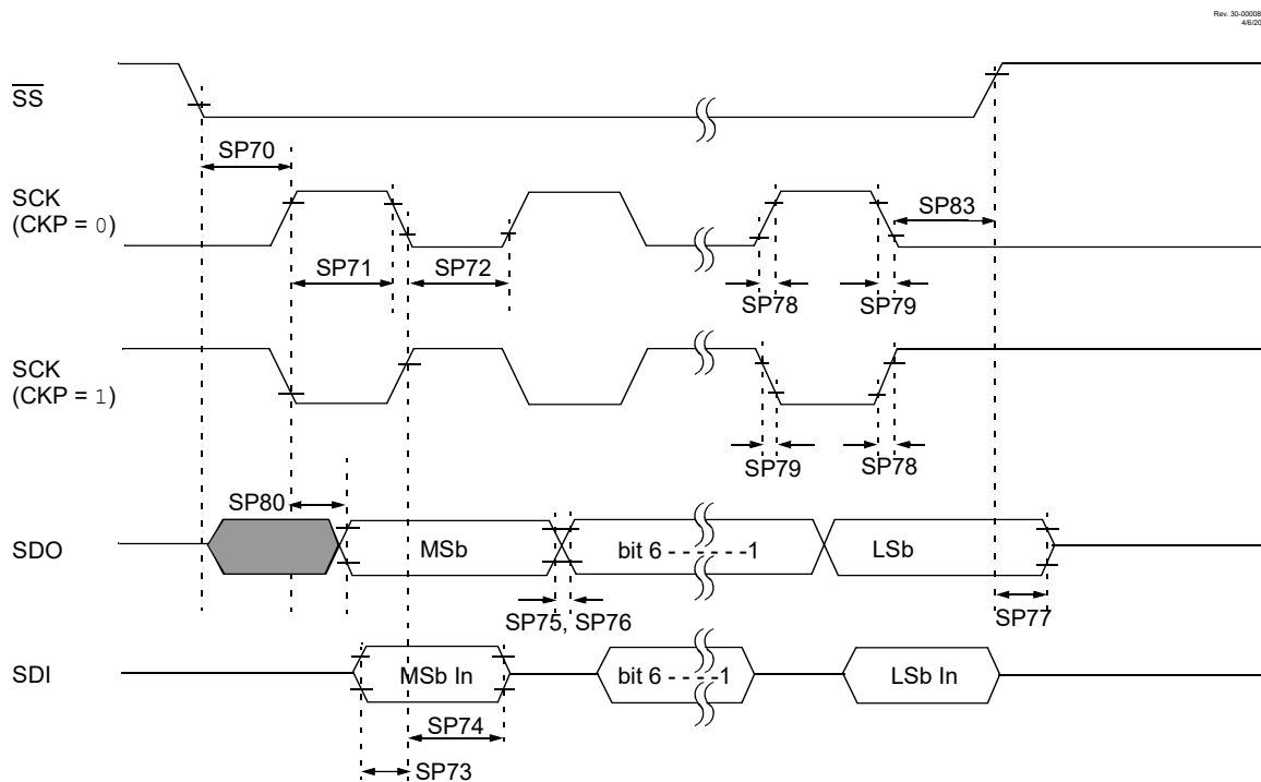
Figure 40-17. SPI Client Mode Timing (CKE = 0)
