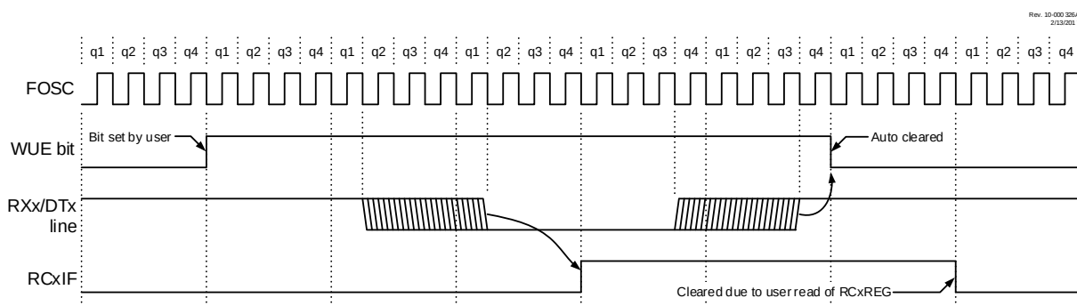
Figure 29-7. Auto-Wake-Up (WUE) Bit Timing During Normal Operation
