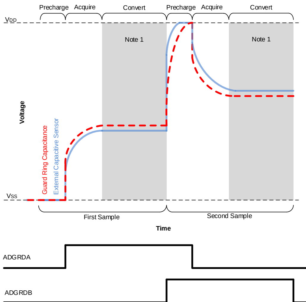
Figure 30-10. Differential CVD with Guard Ring Output Waveform
