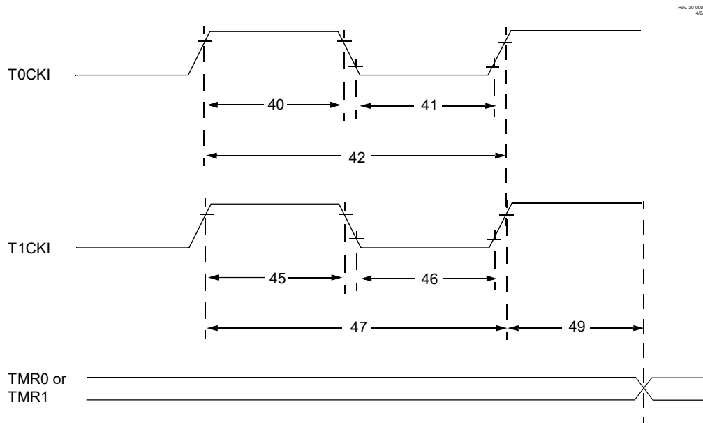
Figure 40-7. Timer0 and Timing1 External Clock Timings
