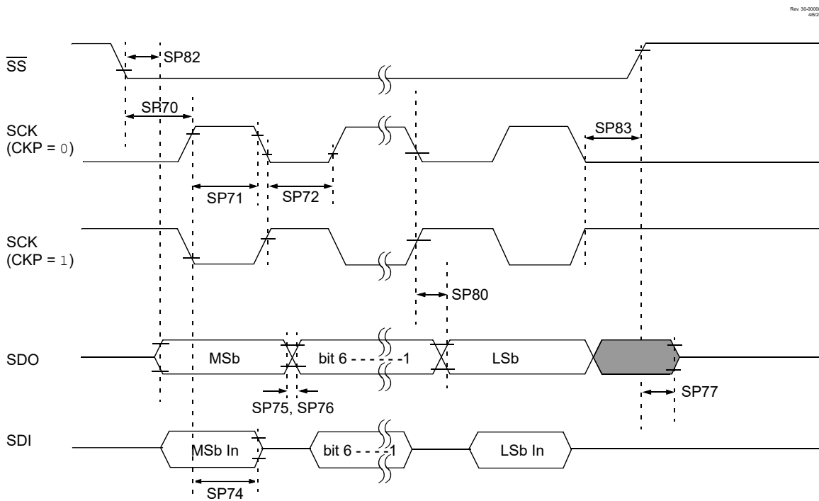
Figure 40-18. SPI Client Mode Timing (CKE = 1)
