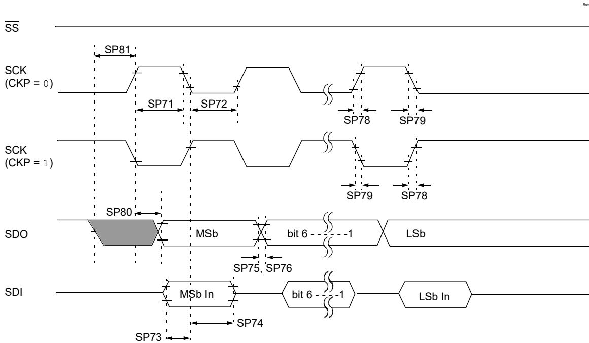
Figure 40-15. SPI Host Mode Timing (CKE = 0, SMP = 0)
