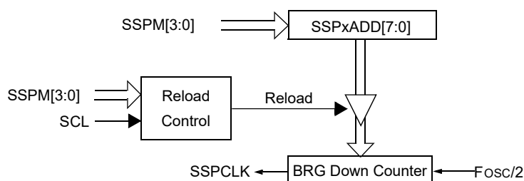
Figure 28-41. Baud Rate Generator Block Diagram
