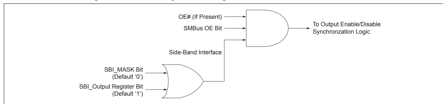
Figure 4. Output Enable Logic (per output)
