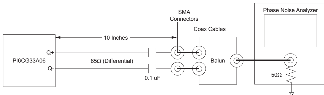
Figure 10. Test Setup for PCIe Jitter Measurement
