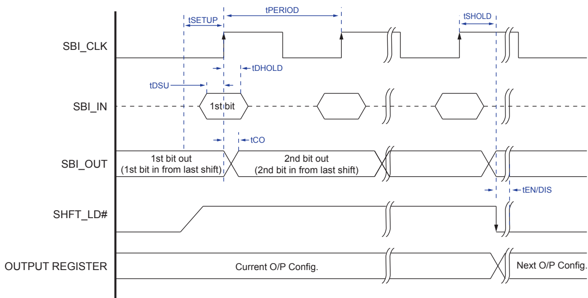
Figure 9. Side Band Interface Timing
