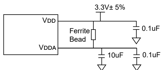
Figure 11. Power Supply Filter
