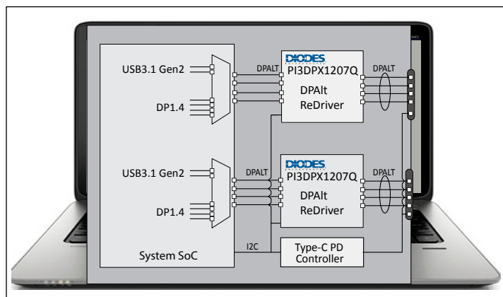
System with Type-C Connector
