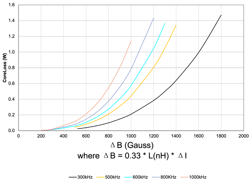
PGL6380.XXXHLT, Core Loss
