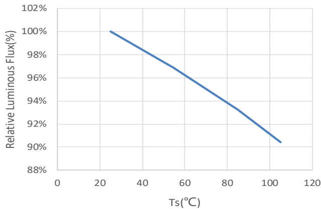
Solder Point Temperature vs. Relative Luminous
