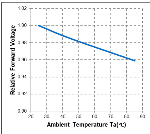
Ambient Temperature vs. Relative Forward Voltage
