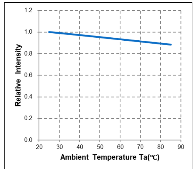
Ambient Temperature vs. Relative Intensity
