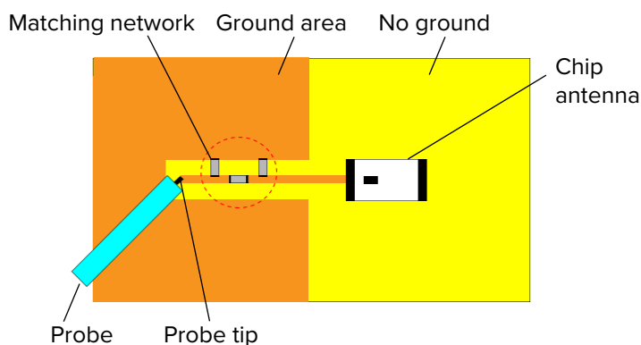
Section of Evaluation Board
