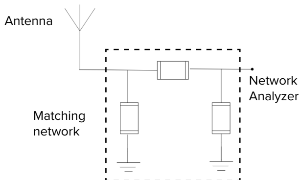
Test Measurement Using Network Analyzer
