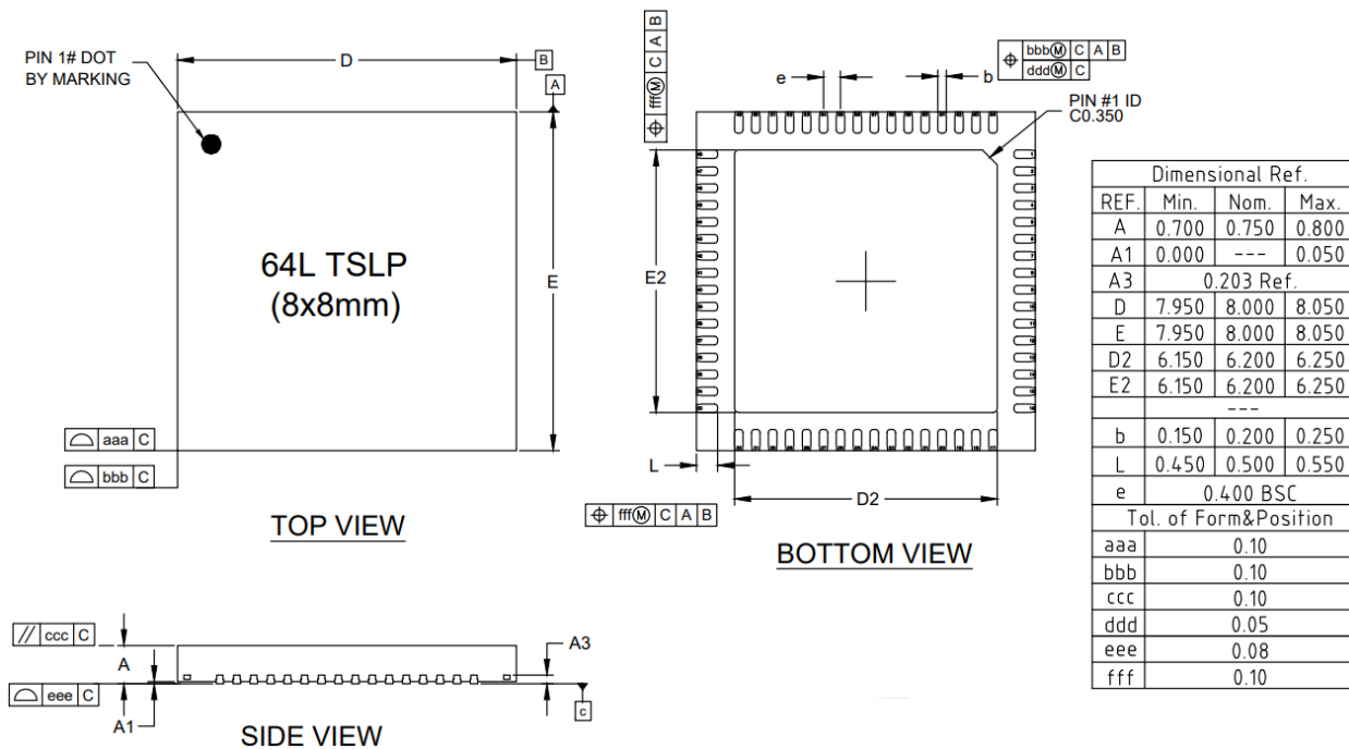
Figure 25-1 TQFN88-64 Package Outline and Dimensions
