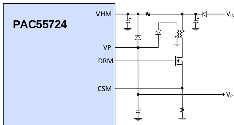
Figure 10-3 SEPIC Mode
