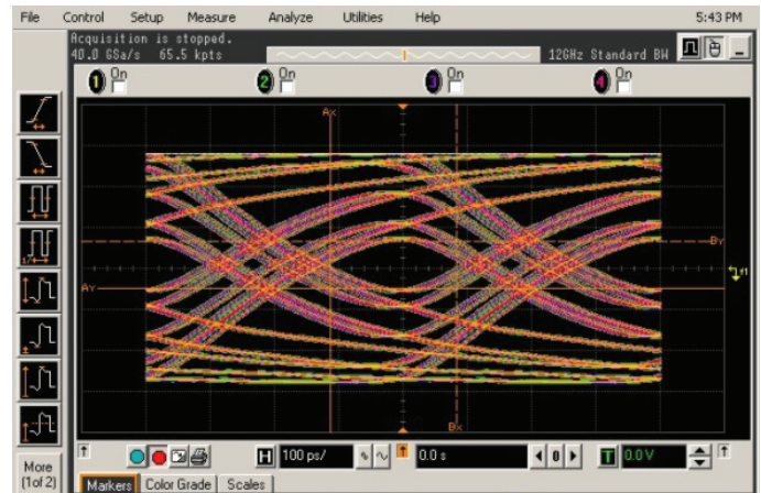
Figure 2: B) Losses from traces, vias, cables, and connectors close the signal eye as it approaches the receiver, increasing the BER substantially and reducing both the reliability and effective throughput of the channel.
