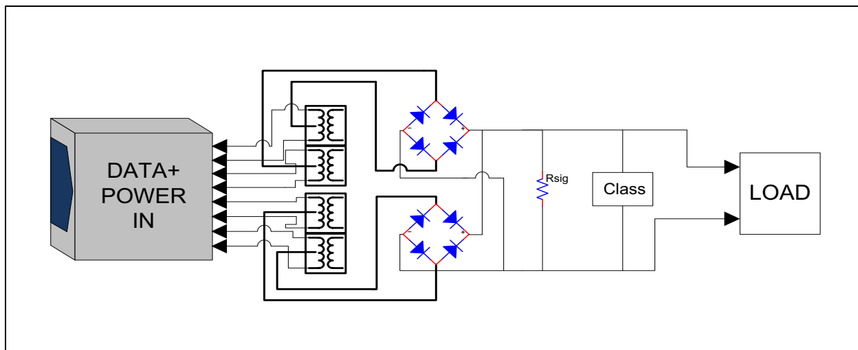
FIGURE 4: DUAL-SIGNATURE PD
