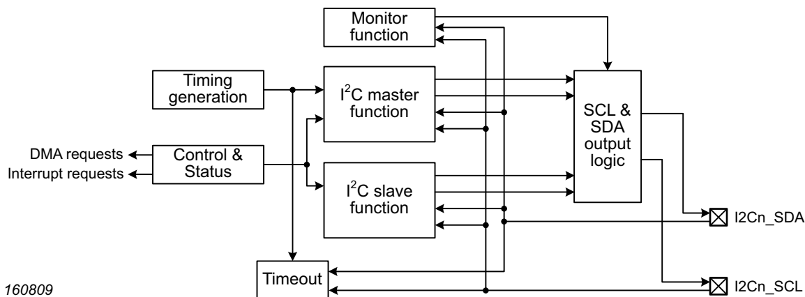
Fig 67. I 2 C block diagram
