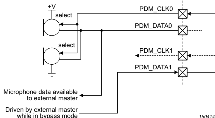
Fig 72. Bypass mode with an external device taking over microphone access
