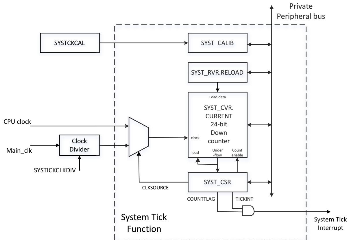
Fig 58. System tick timer block diagram
