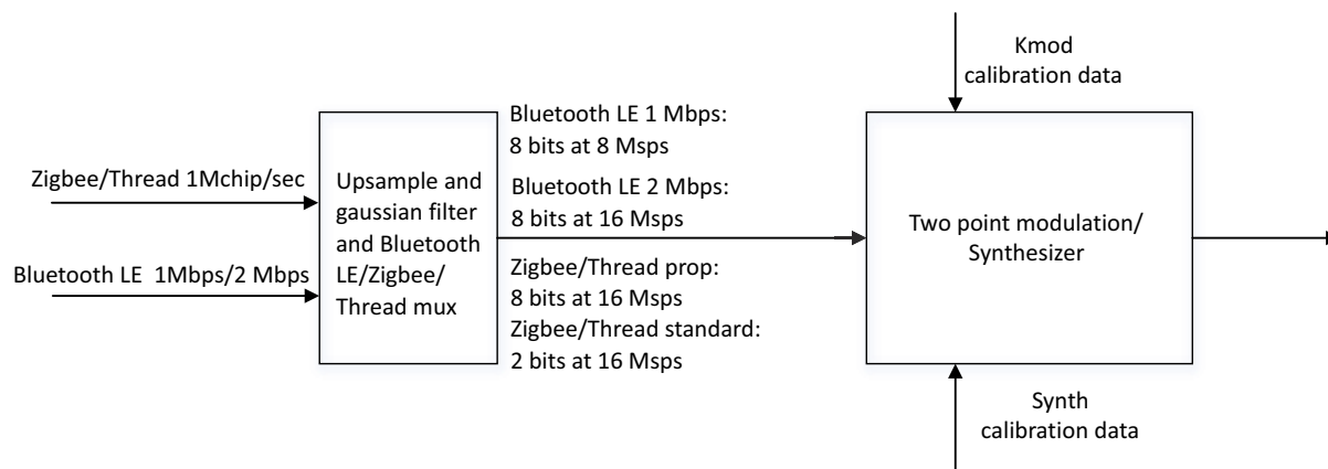
Fig 114. Transmit Datapath architecture
