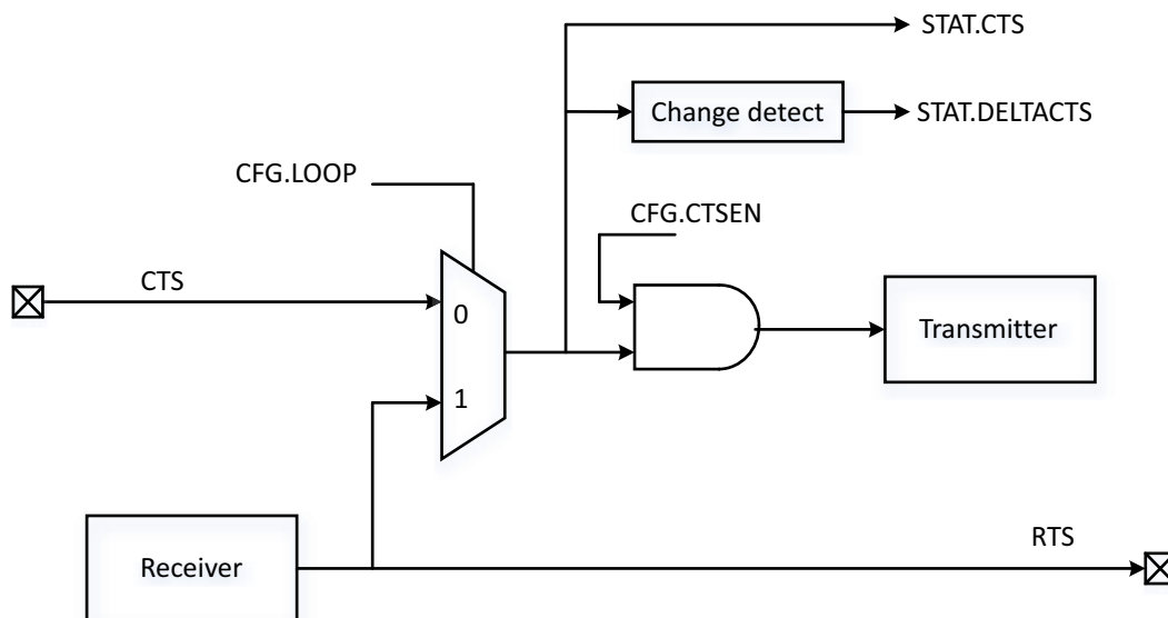
Fig 60. Hardware flow control using RTS and CTS
