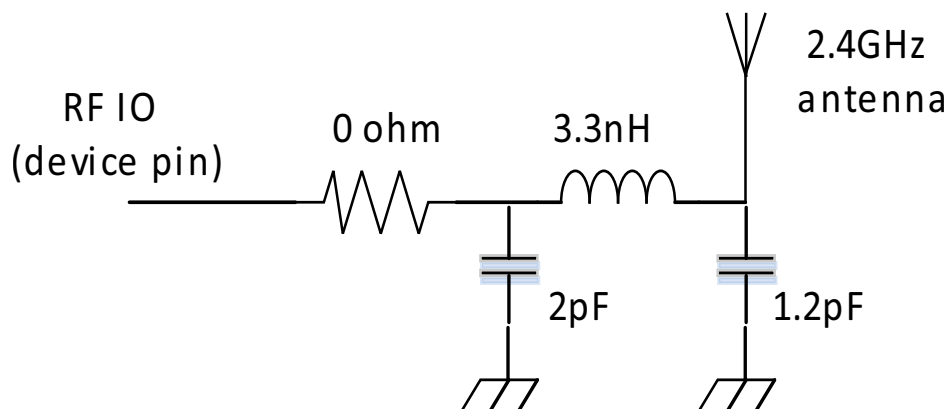
Fig 109. RF matching circuit
