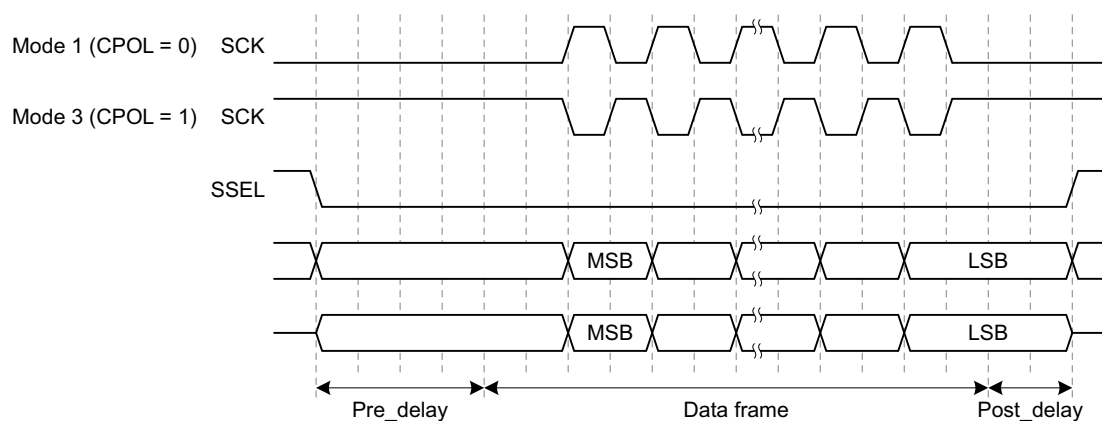
Fig 63. Pre_delay and Post_delay
