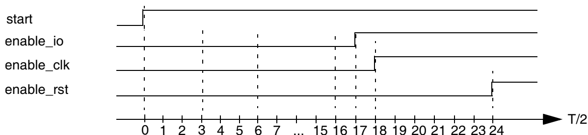
Fig 91. Activation Sequence
