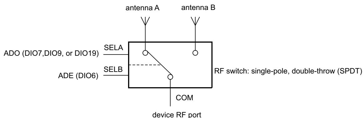
Fig 143. Simple antenna diversity implementation using external RF switch
