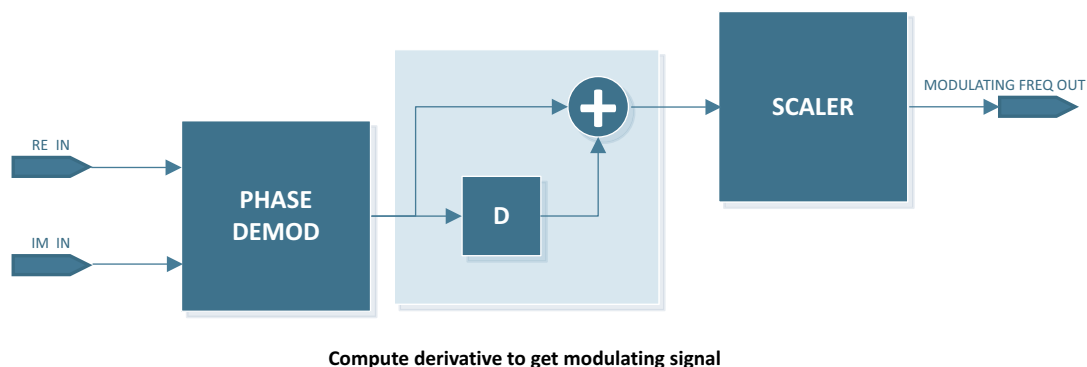
Fig 129. FM demodulator architecture
