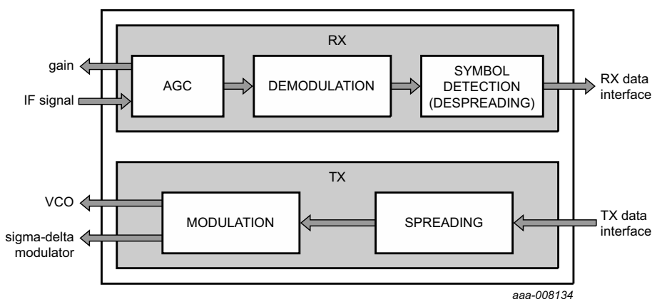
Fig 119. Modem architecture
