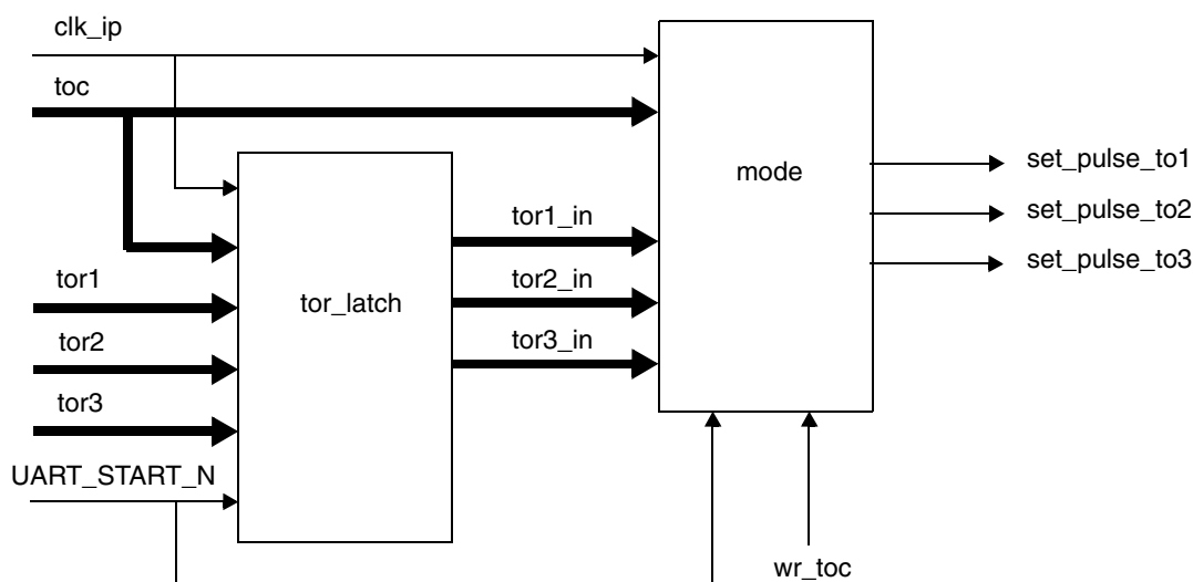
Fig 94. Timer block diagram
