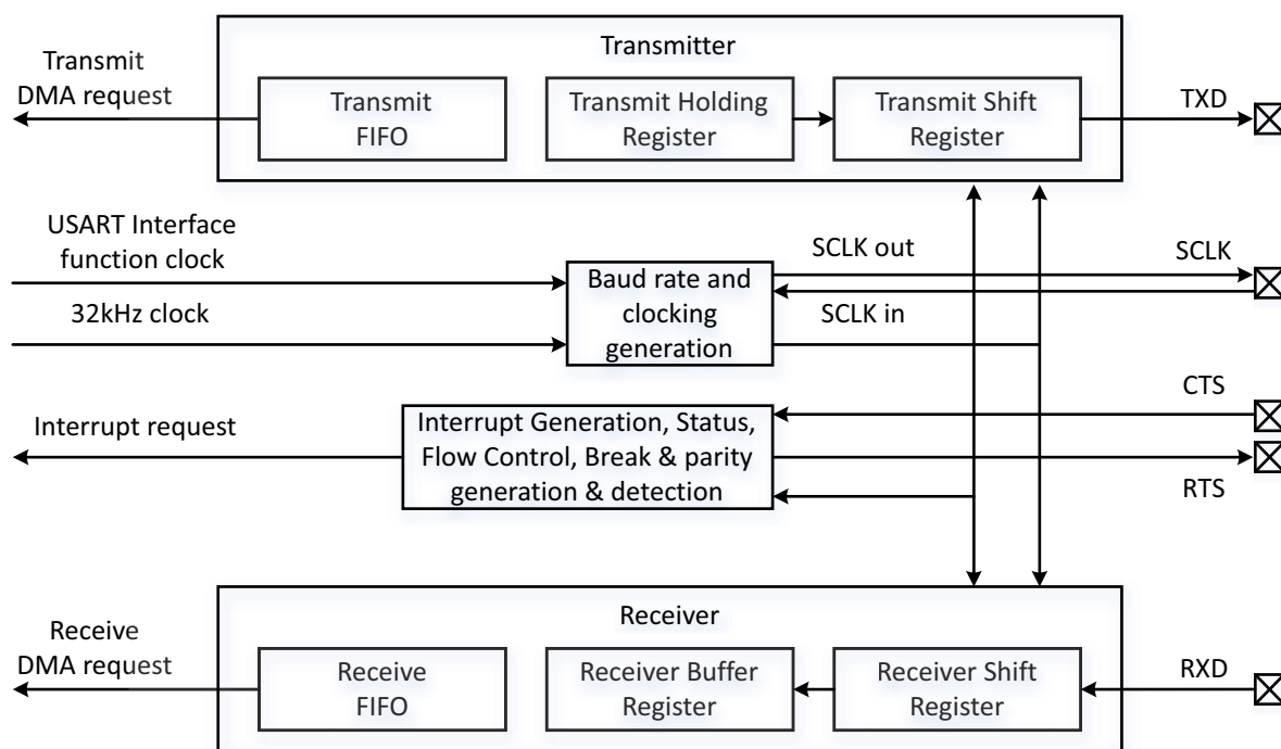
Fig 59. USART block diagram
