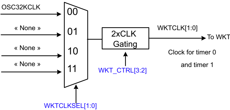
Fig 19. WKT clock selection and gating
