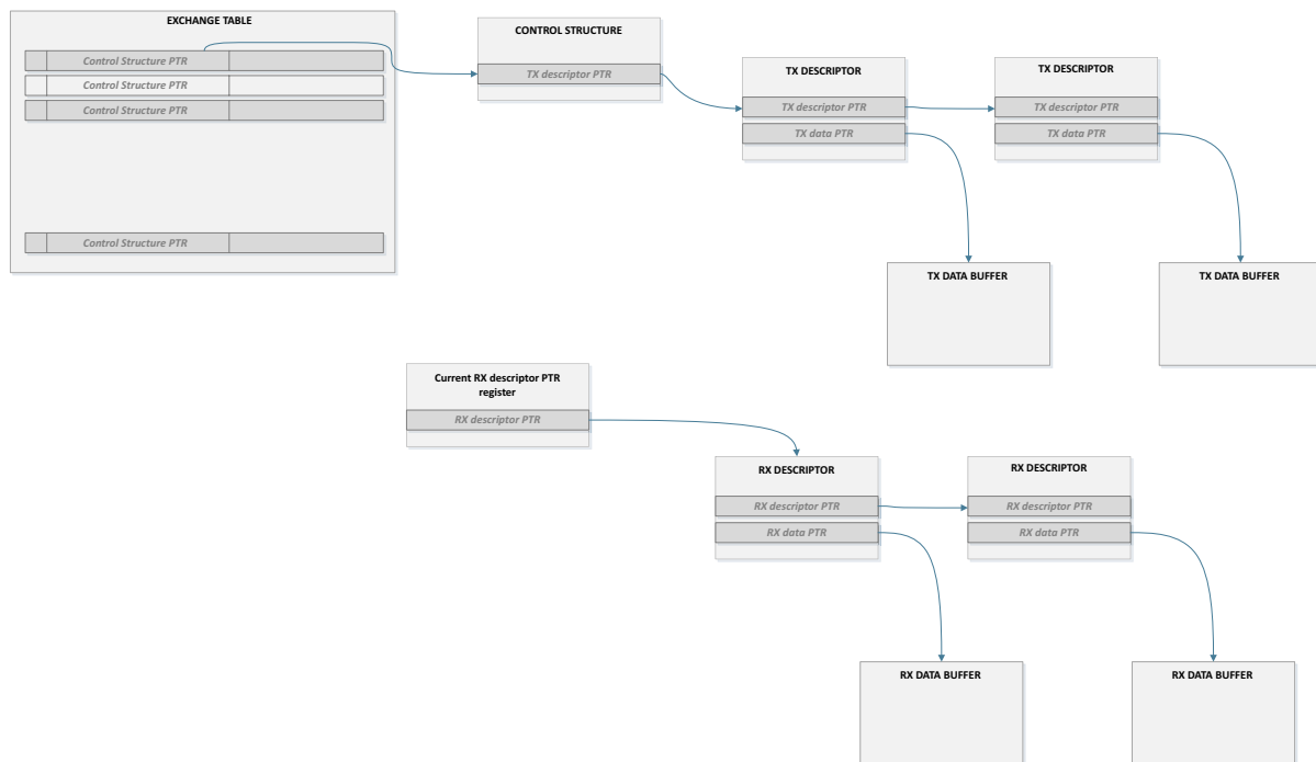
Fig 126. LL software tables
