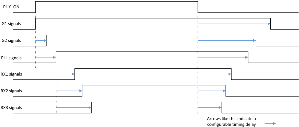
Fig 112. Receive sequence of group enables
