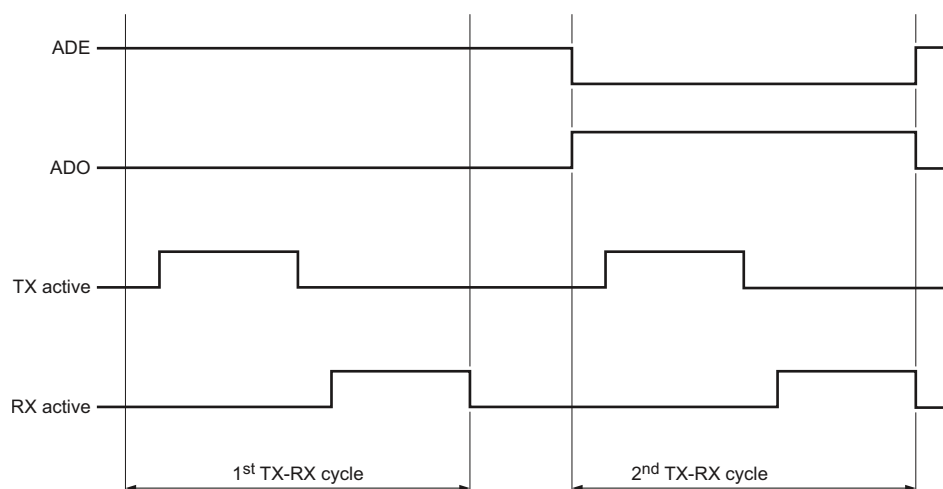
Fig 144. Zigbee/Thread antenna diversity ADO and ADE signals for TX with acknowledgement
