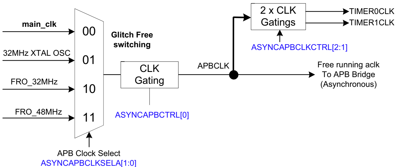
Fig 10. APB clock generation
