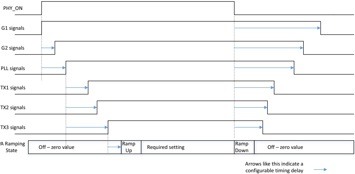
Fig 113. Transmit sequence of group enables
