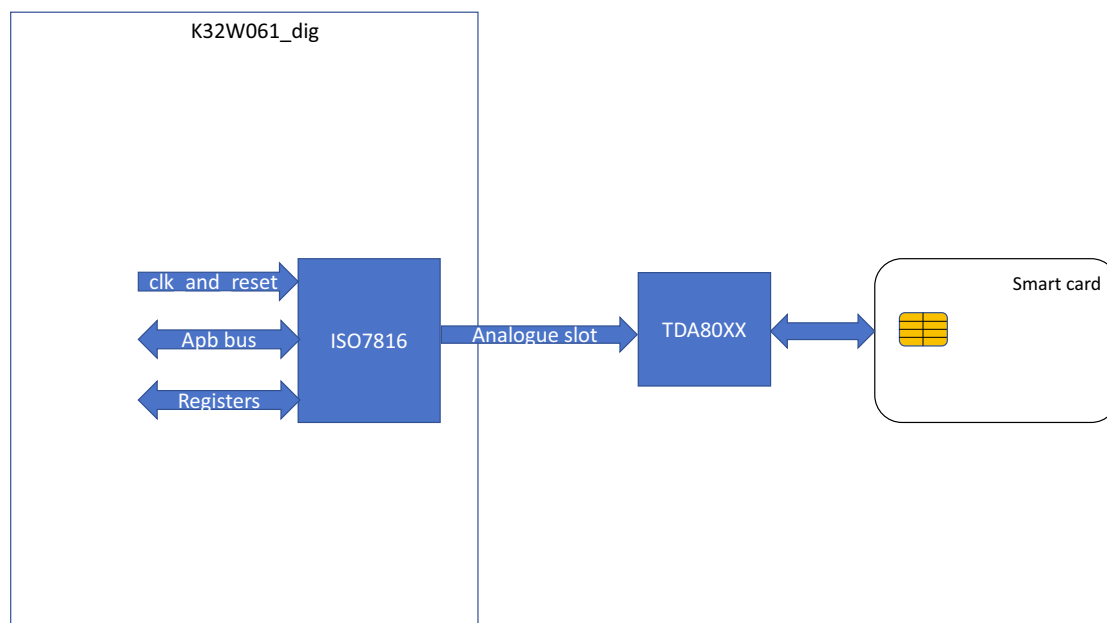
Fig 97. ISO7816 interface
