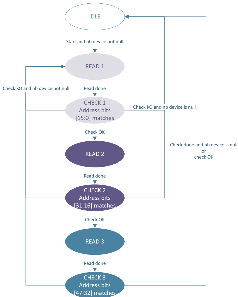
Fig 139. White list engine state machine
