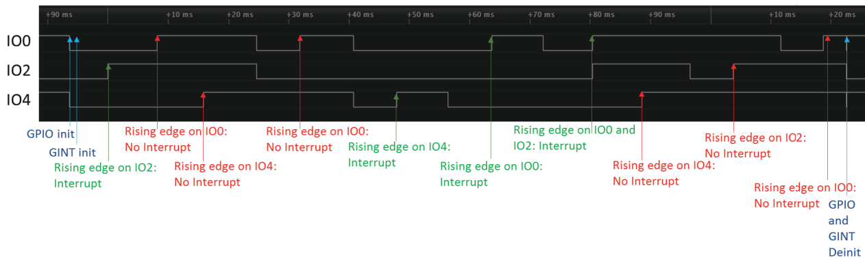
Fig 41. GINT Example for "(IO0 asserted) OR (IO2 asserted) OR (IO4 asserted)"
