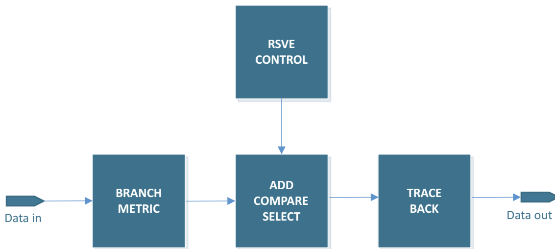
Fig 134. Reduced State Viterbi Equaliser
