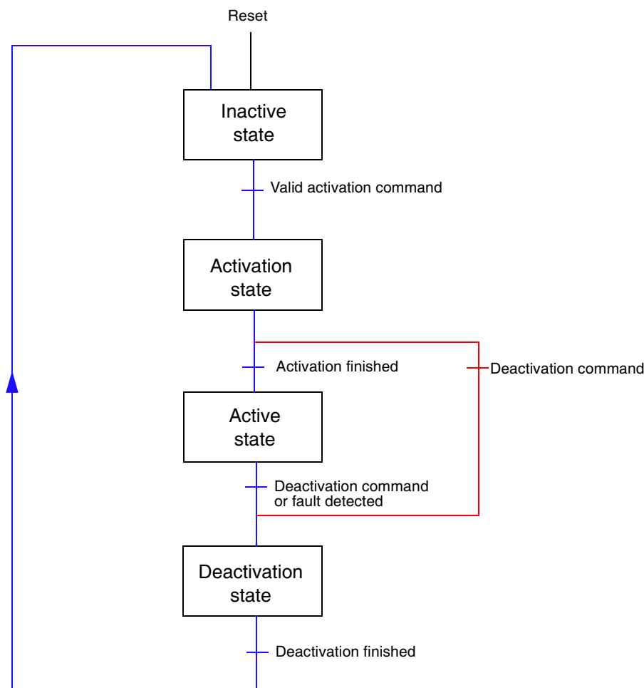
Fig 90. Sequencer FSM block diagram
