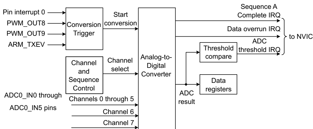
Fig 83. ADC block diagram
