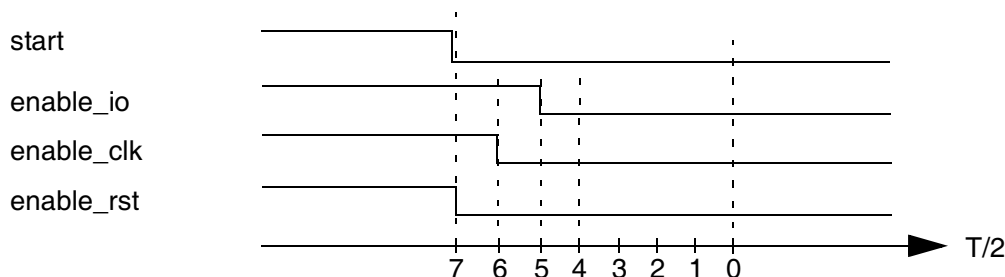
Fig 92. Deactivation Sequence
