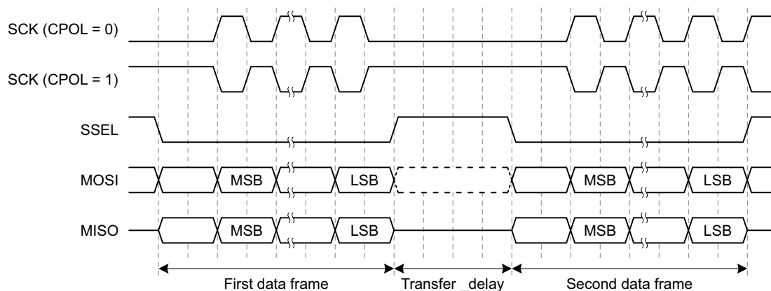
Fig 65. Transfer_delay
