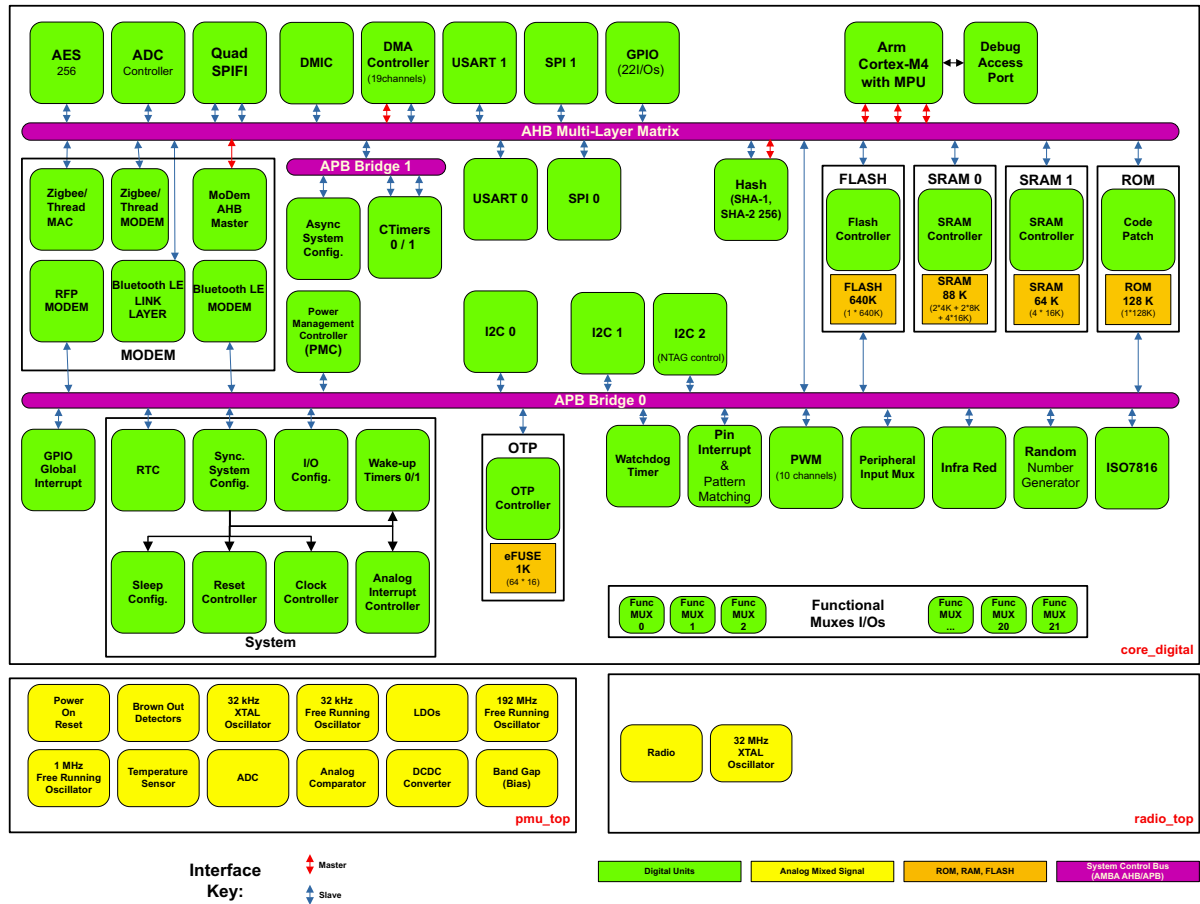
Fig 1. Chip block diagram
