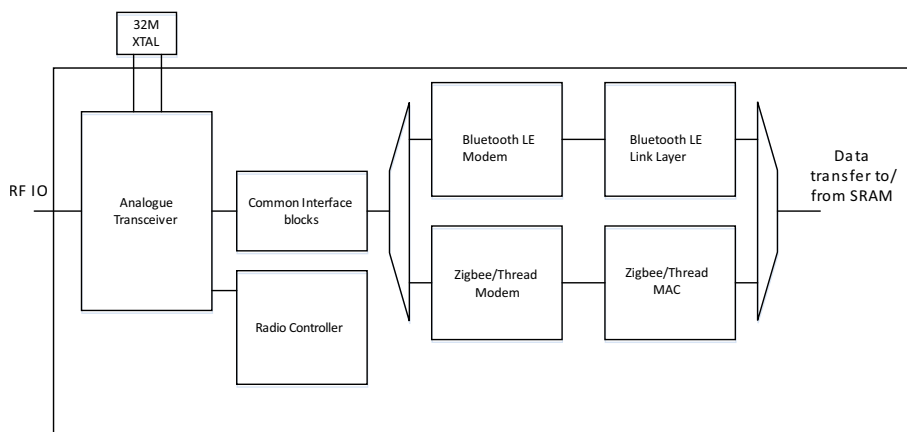
Fig 109. Radio system block diagram
