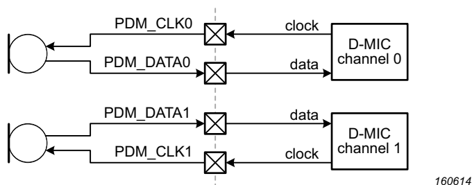
Fig 71. Typical connection to two independent microphones
