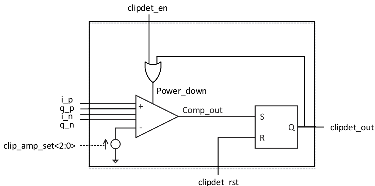
Fig 120. Clip detector 2
