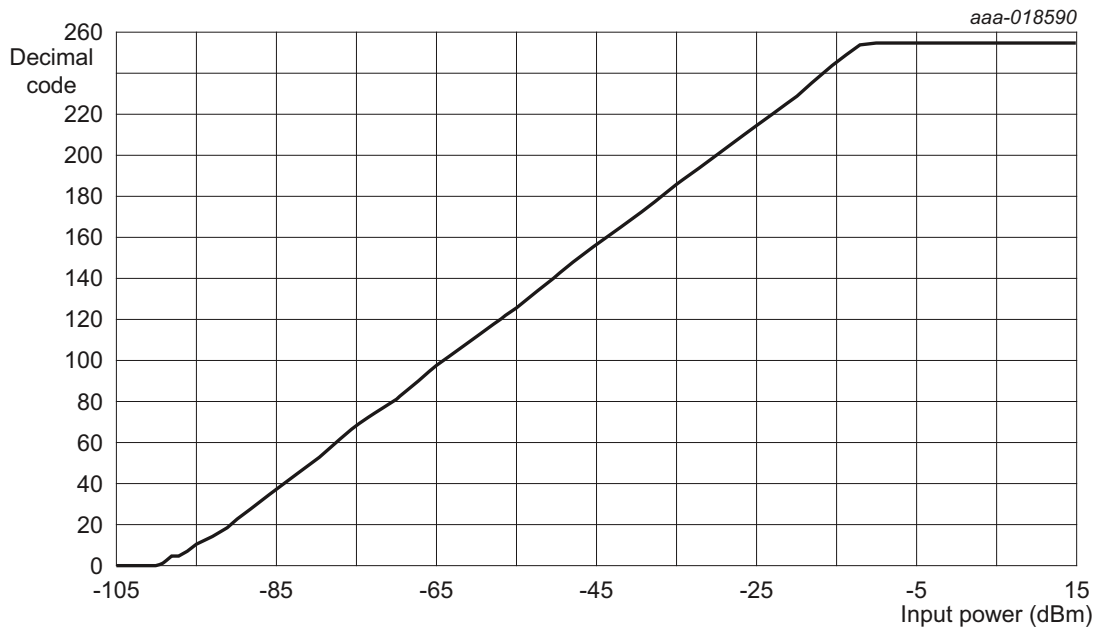
Fig 122. Energy detect (ED) value versus input power level
