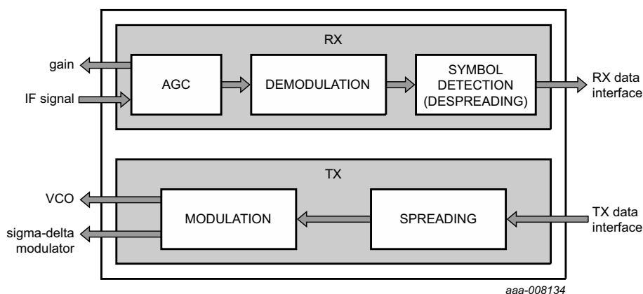
Fig 121. Modem architecture
