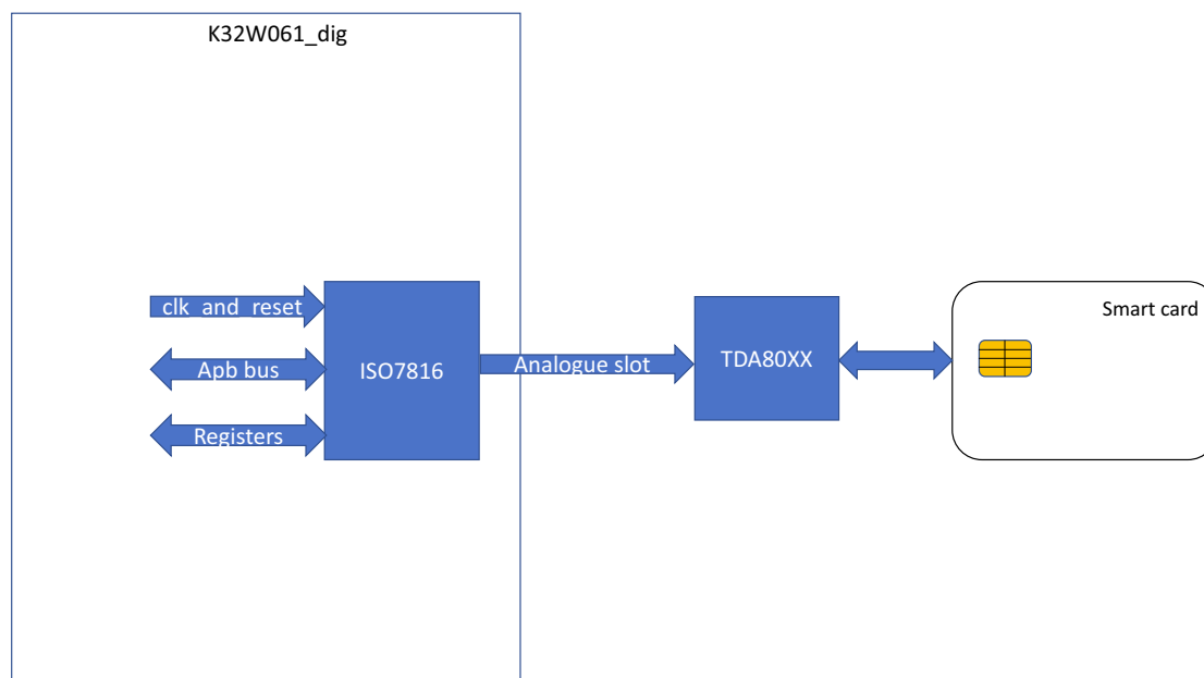
Fig 99. ISO7816 interface
