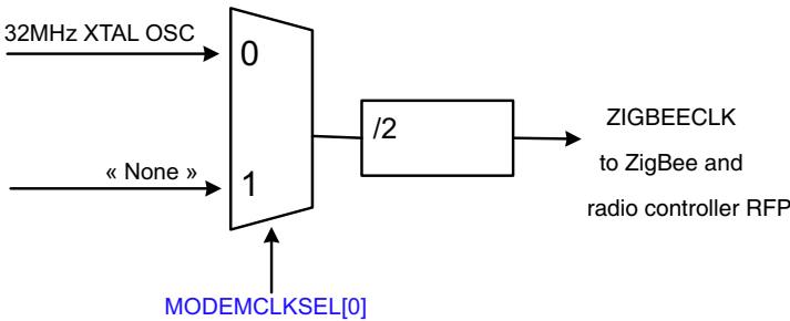
Fig 18. Zigbee/Thread clock selection
