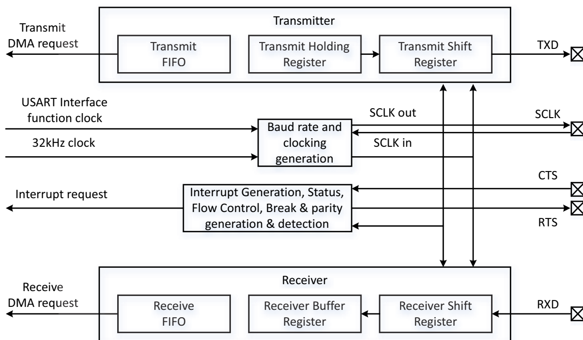
Fig 61. USART block diagram
