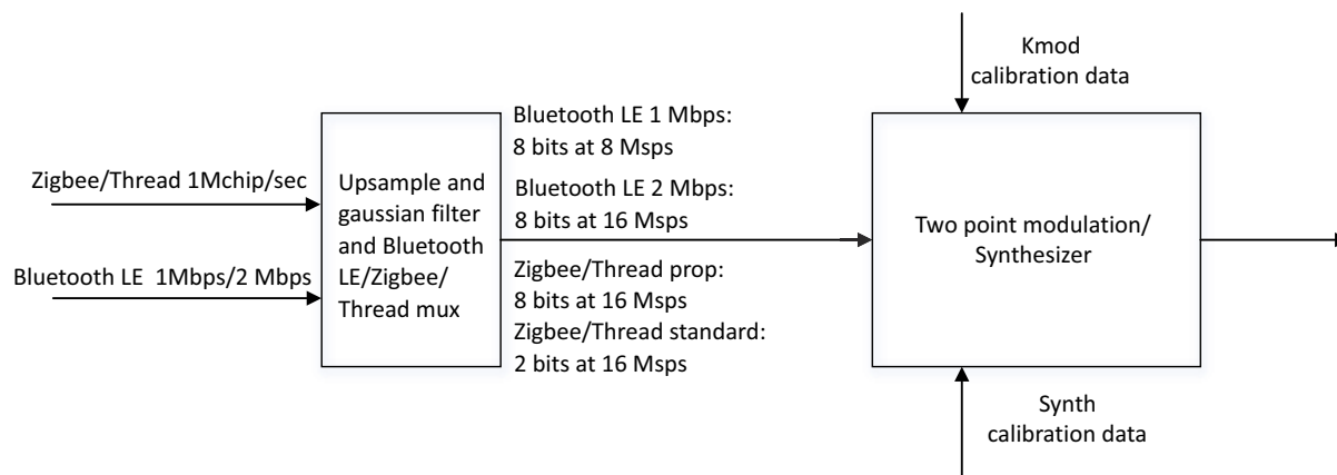
Fig 116. Transmit Datapath architecture
