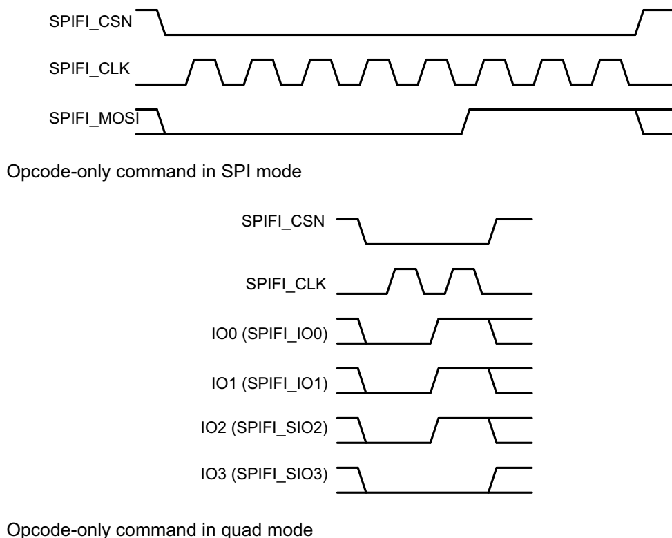
Fig 89. Opcode only commands
