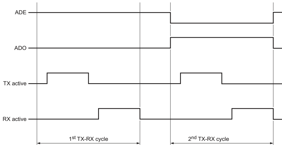
Fig 146. Zigbee/Thread antenna diversity ADO and ADE signals for TX with acknowledgment
