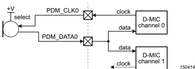
Fig 73. Typical connection to a stereo microphone
