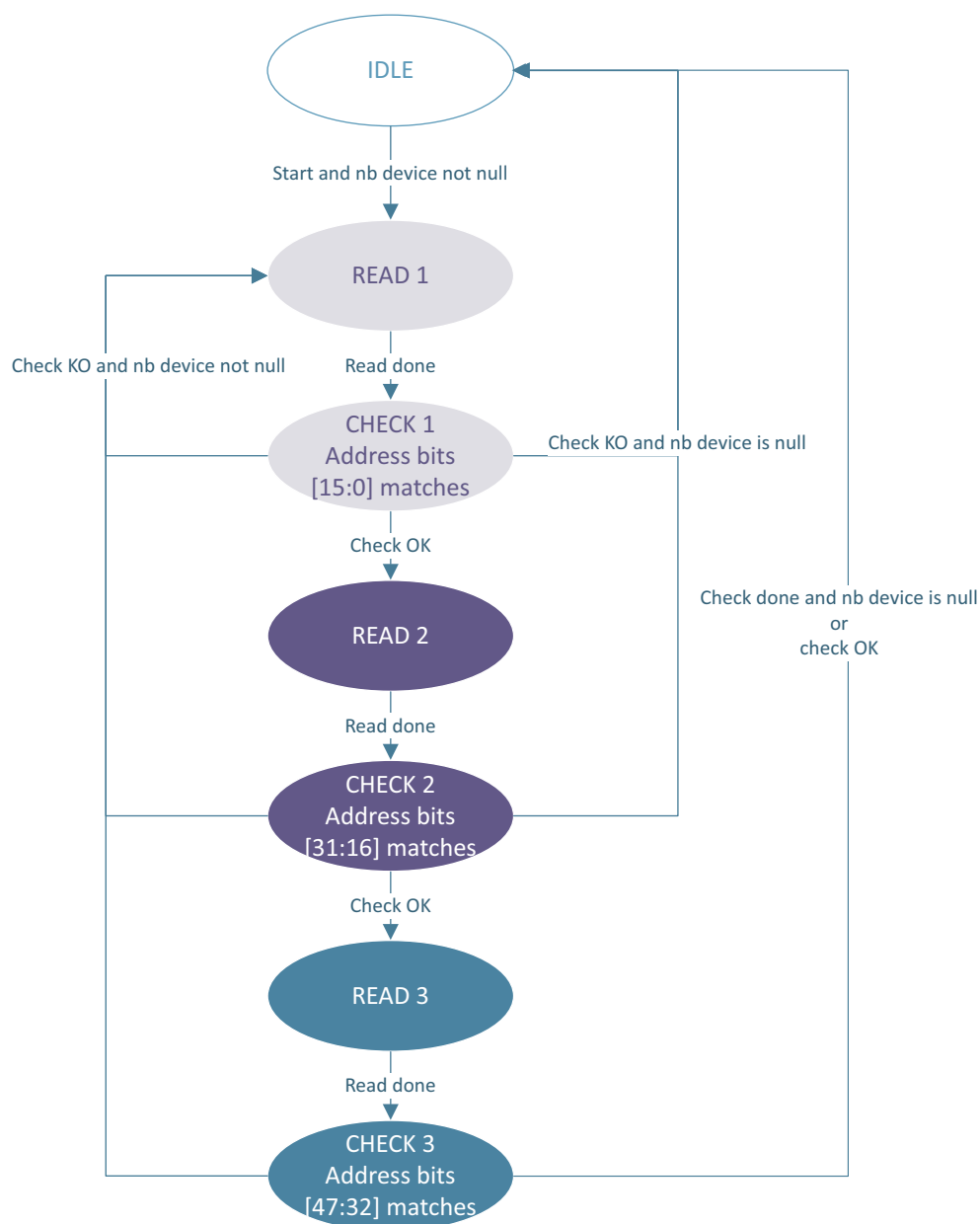
Fig 141. White list engine state machine
