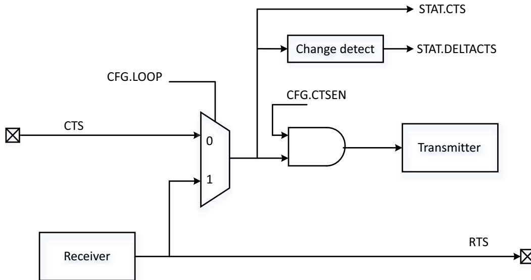
Fig 62. Hardware flow control using RTS and CTS
