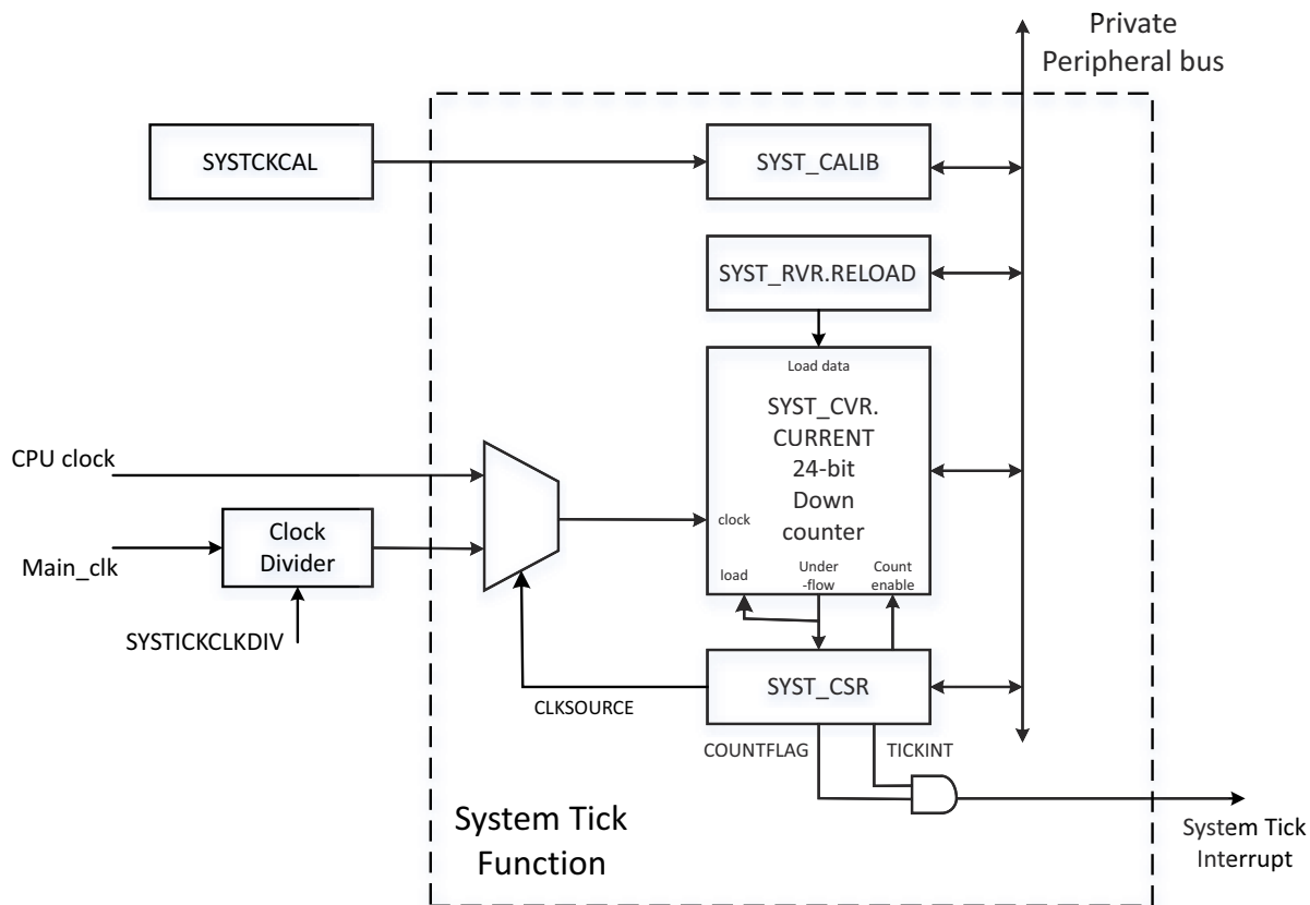
Fig 60. System tick timer block diagram
