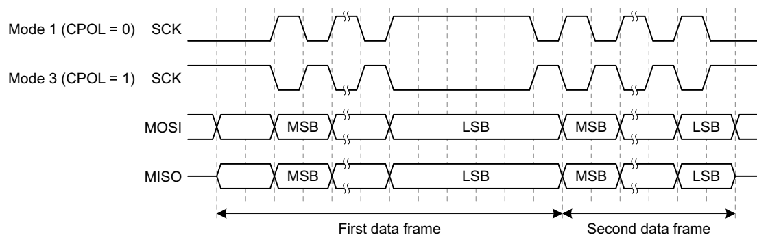
Fig 68. Examples of data stalls
