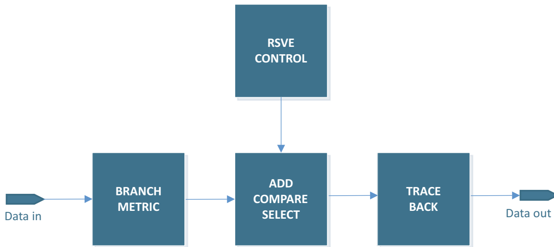
Fig 136. Reduced State Viterbi Equaliser
