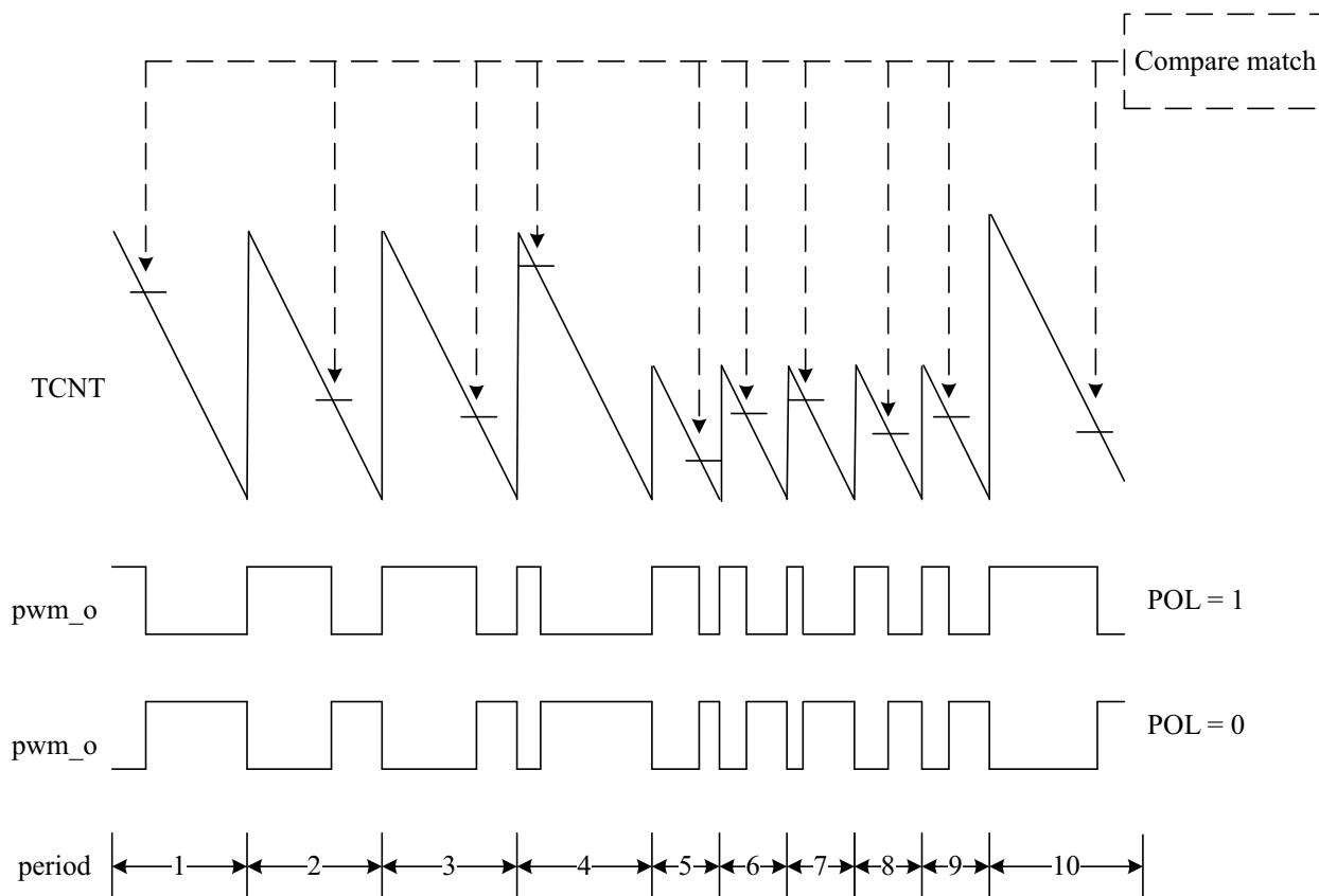
Fig 49. PWM Waveform
