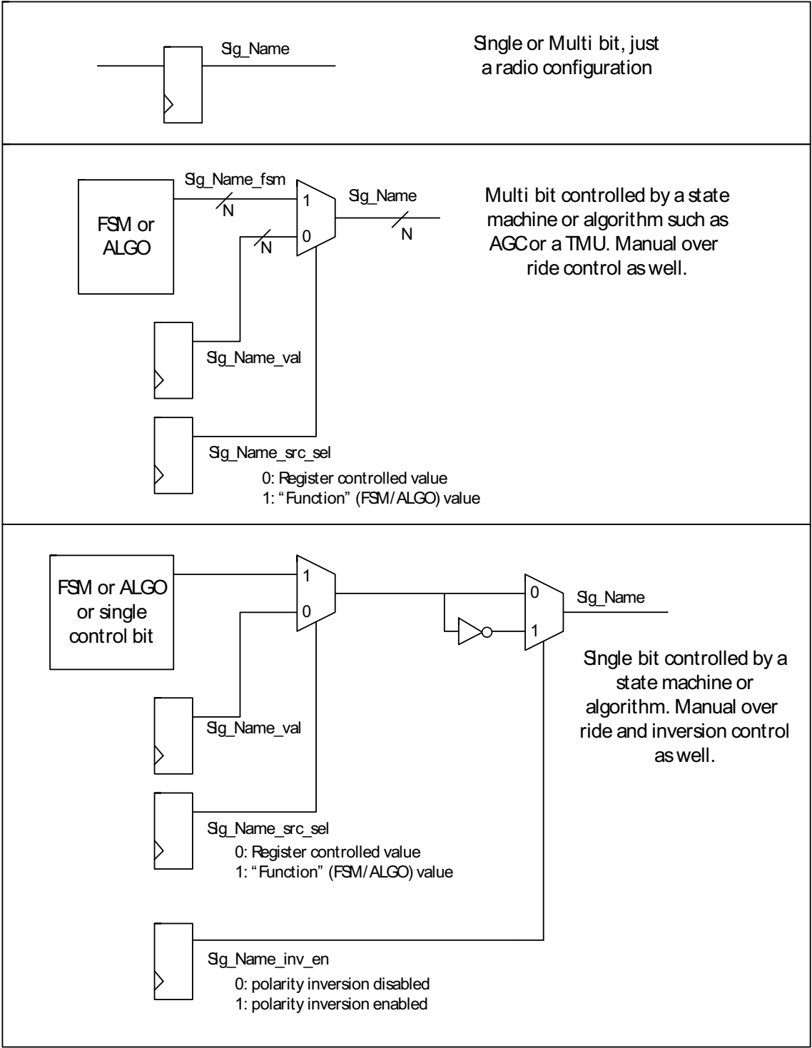
Fig 112. Radio interface control configuration
