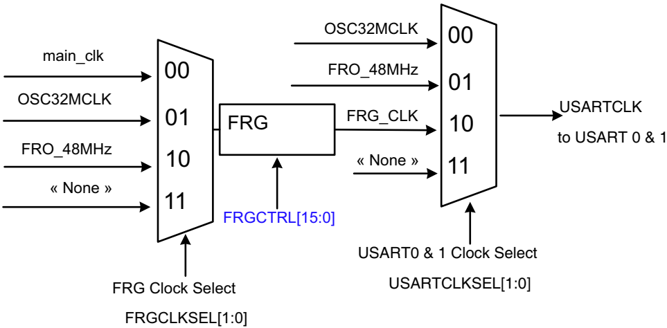
Fig 16. USART clocks selection
