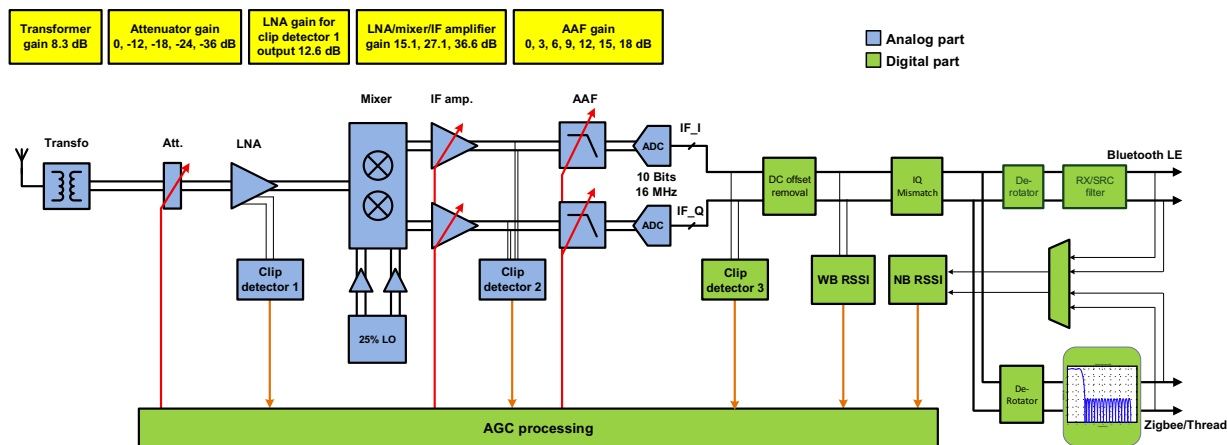
Fig 118. Receiver simplified block diagram for AGC
