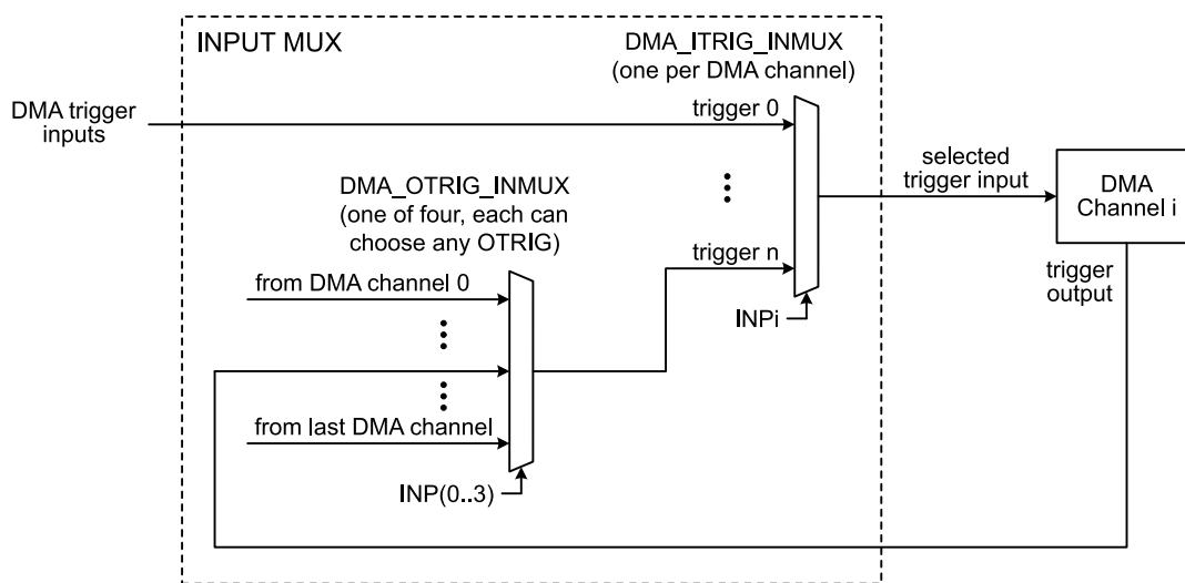
Fig 35. DMA trigger multiplexing
