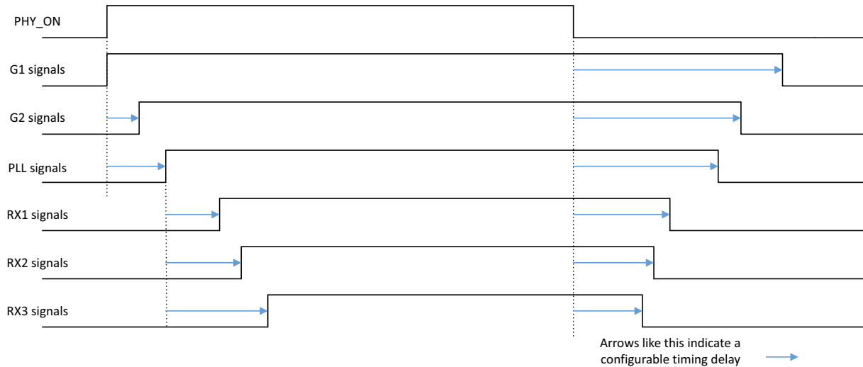
Fig 114. Receive sequence of group enables
