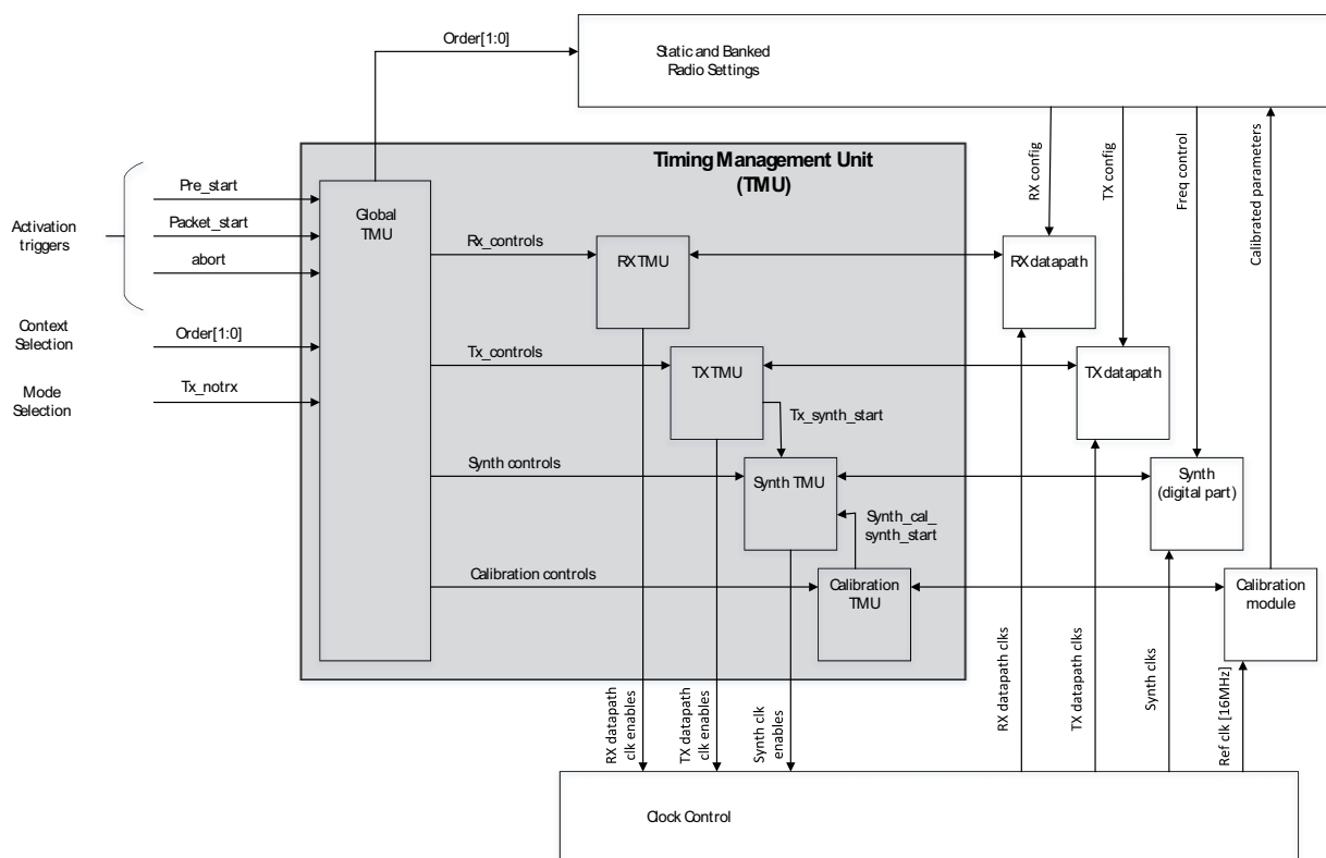
Fig 113. TMU architecture
