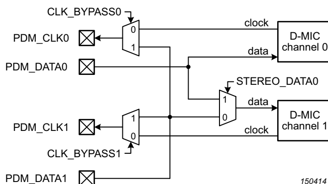
Fig 70. DMIC subsystem pin multiplexing
