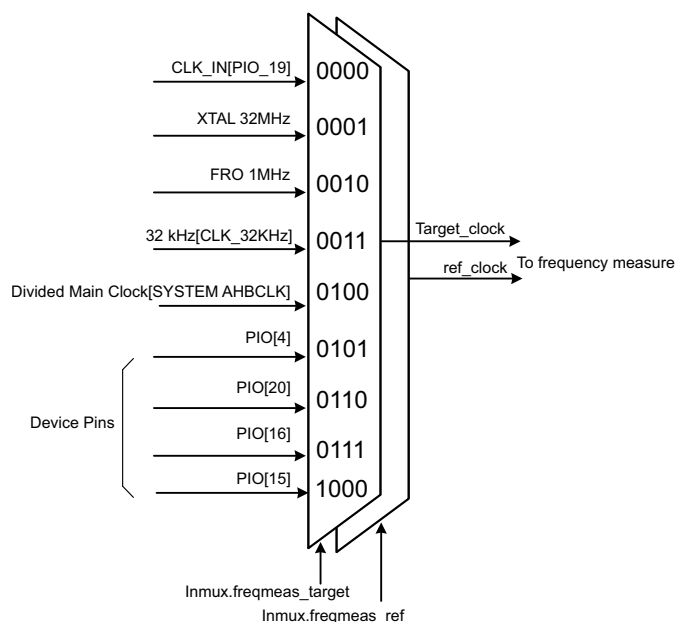
Fig 101. Clock sources to frequency measure block diagram
