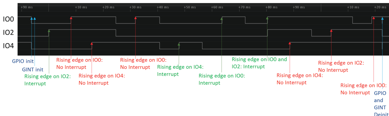
Fig 43. GINT Example for “(IO0 asserted) OR (IO2 asserted) OR (IO4 asserted)”
