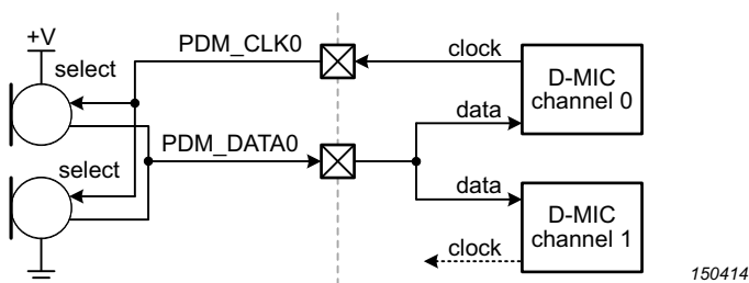
Fig 72. Typical connection to two microphones sharing a data line
