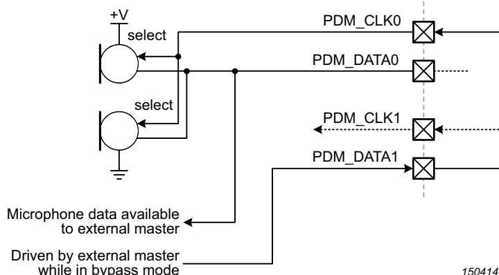
Fig 74. Bypass mode with an external device taking over microphone access
