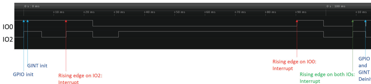
Fig 44. GINT example for “(IO0 asserted) AND (IO2 asserted)”
