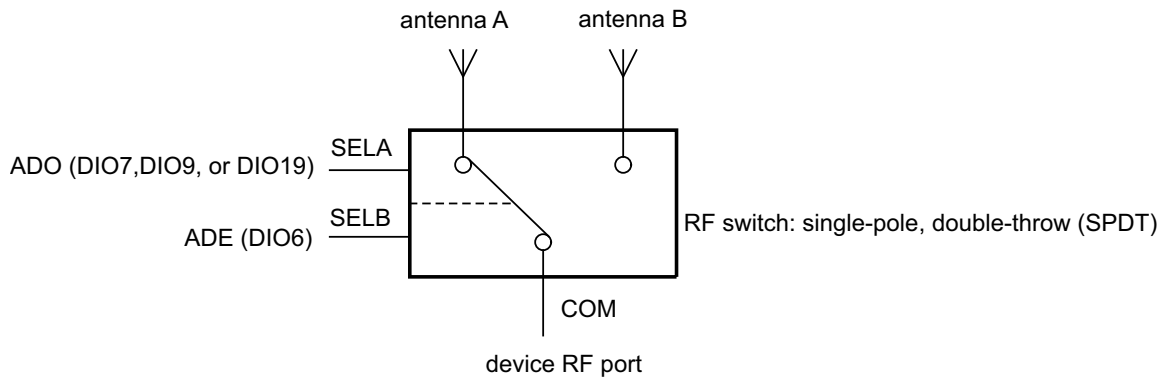
Fig 145. Simple antenna diversity implementation using external RF switch
