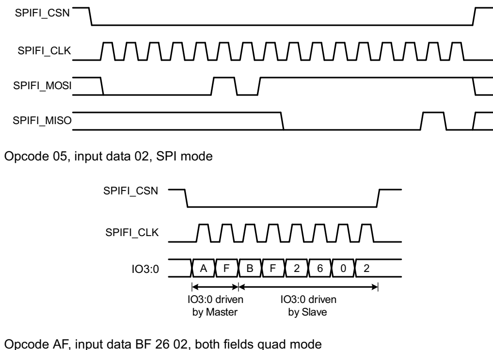
Fig 90. Read commands
