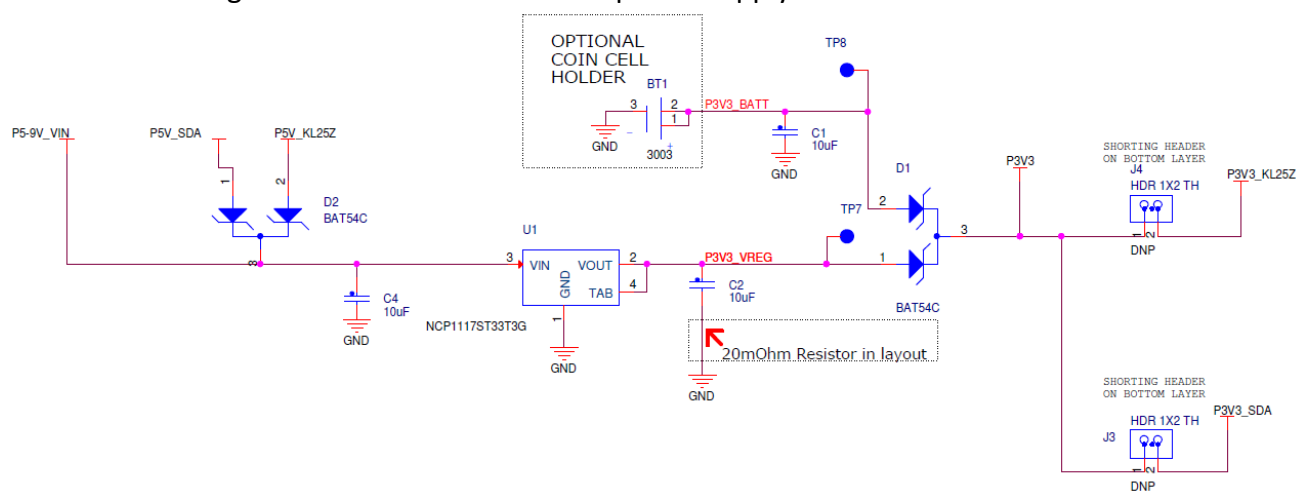
Figure A-1. Power Supply Schematic Rev. D.
