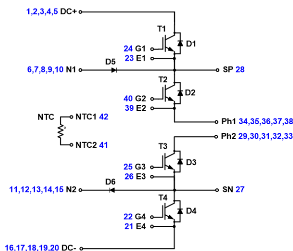
Figure 1. NXH350N100H4Q2F2P1G/S1G Schematic Diagram
