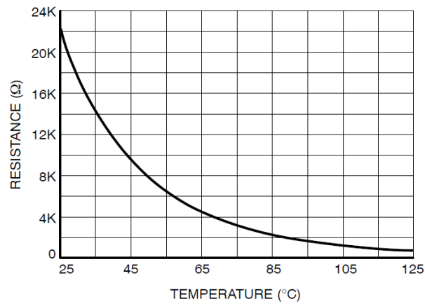
Figure 51. Thermistor Characteristics
