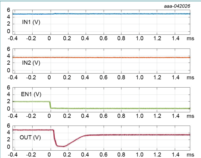
Fig. 27. OR-ing with enable ( V_{IN1} = 5 V , V_{IN2} = 3.6 V ; EN1 High to Low transition, EN2 tied to V_{IN2} )
