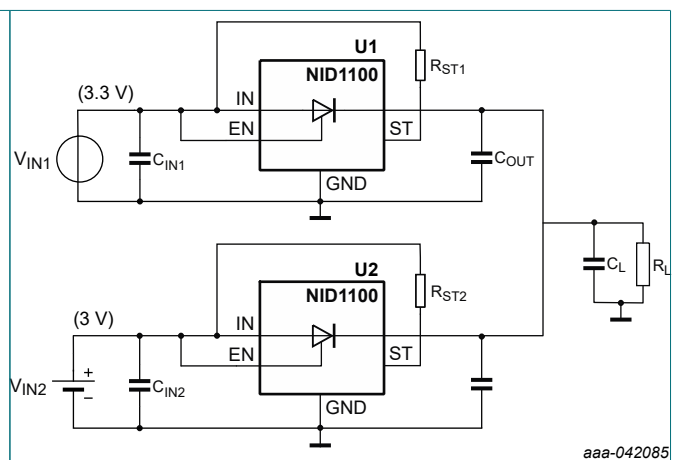
Fig. 35. OR-ing with NID1100
