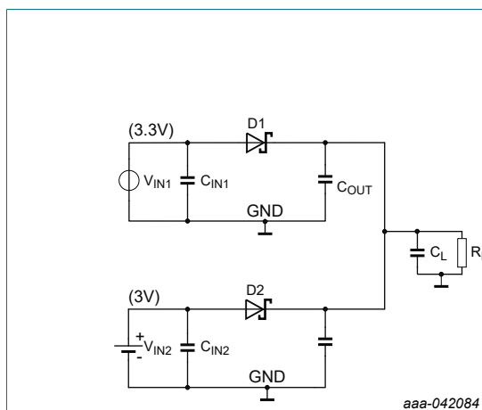
Fig. 34. OR-ing with Schottky diodes
