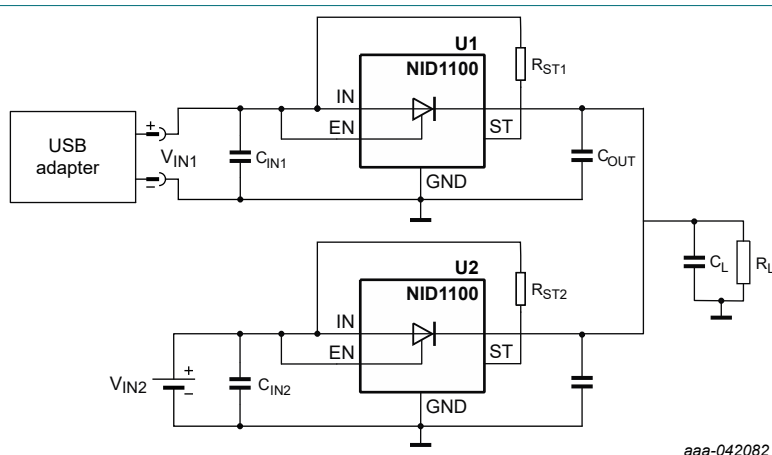
Fig. 32. OR-ing power supply and battery
