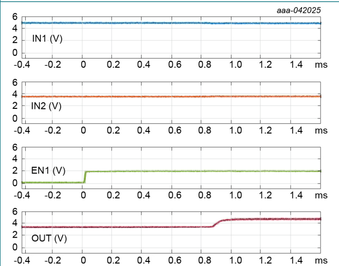
Fig. 26. OR-ing with enable ( V_{IN1} = 5 V , V_{IN2} = 3.6 V ; EN1 Low to High transition, EN2 tied to V_{IN2} )
