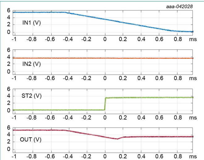
Fig. 29. OR-ing with V_{IN} ( V_{IN1} = 5\text{ V} to 0\text{ V} in 1\text{ ms} , V_{IN2} = 3.6\text{ V} ; EN1 tied to V_{IN1} , EN2 tied to V_{IN2} )
