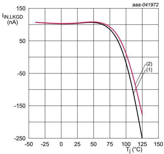
Fig. 12. Input leakage current, disabled, ( I_{IN,LKGD} ) versus junction temperature at V_{OUT} = 5 V
