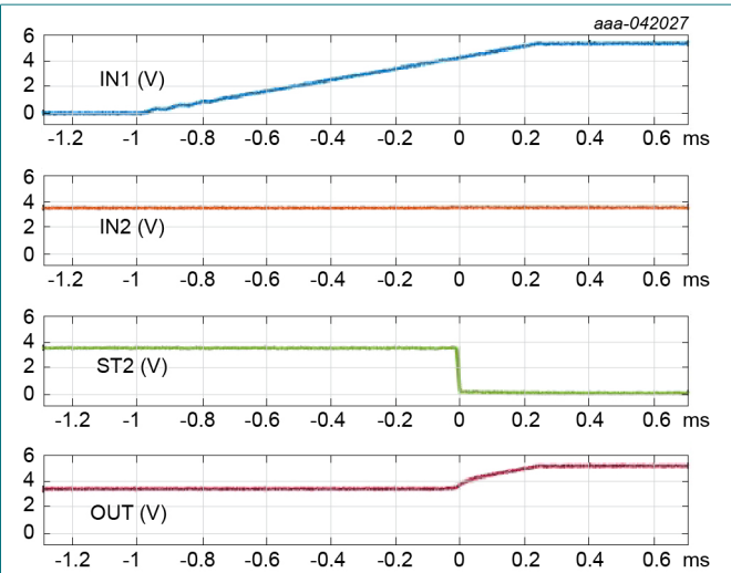
Fig. 28. FOR-ing with V_{IN} ( V_{IN1} = 0\text{ V} to 5\text{ V} in 1\text{ ms} , V_{IN2} = 3.6\text{ V} ; EN1 tied to V_{IN1} , EN2 tied to V_{IN2} )
