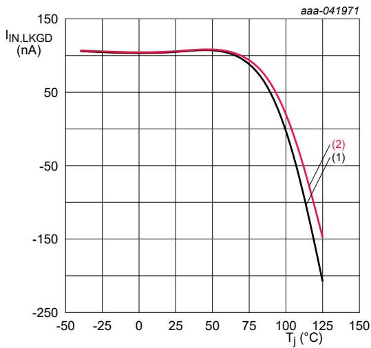
Fig. 11. Input leakage current, disabled, ( I_{IN,LKGD} ) versus junction temperature at V_{OUT} = 4 V
