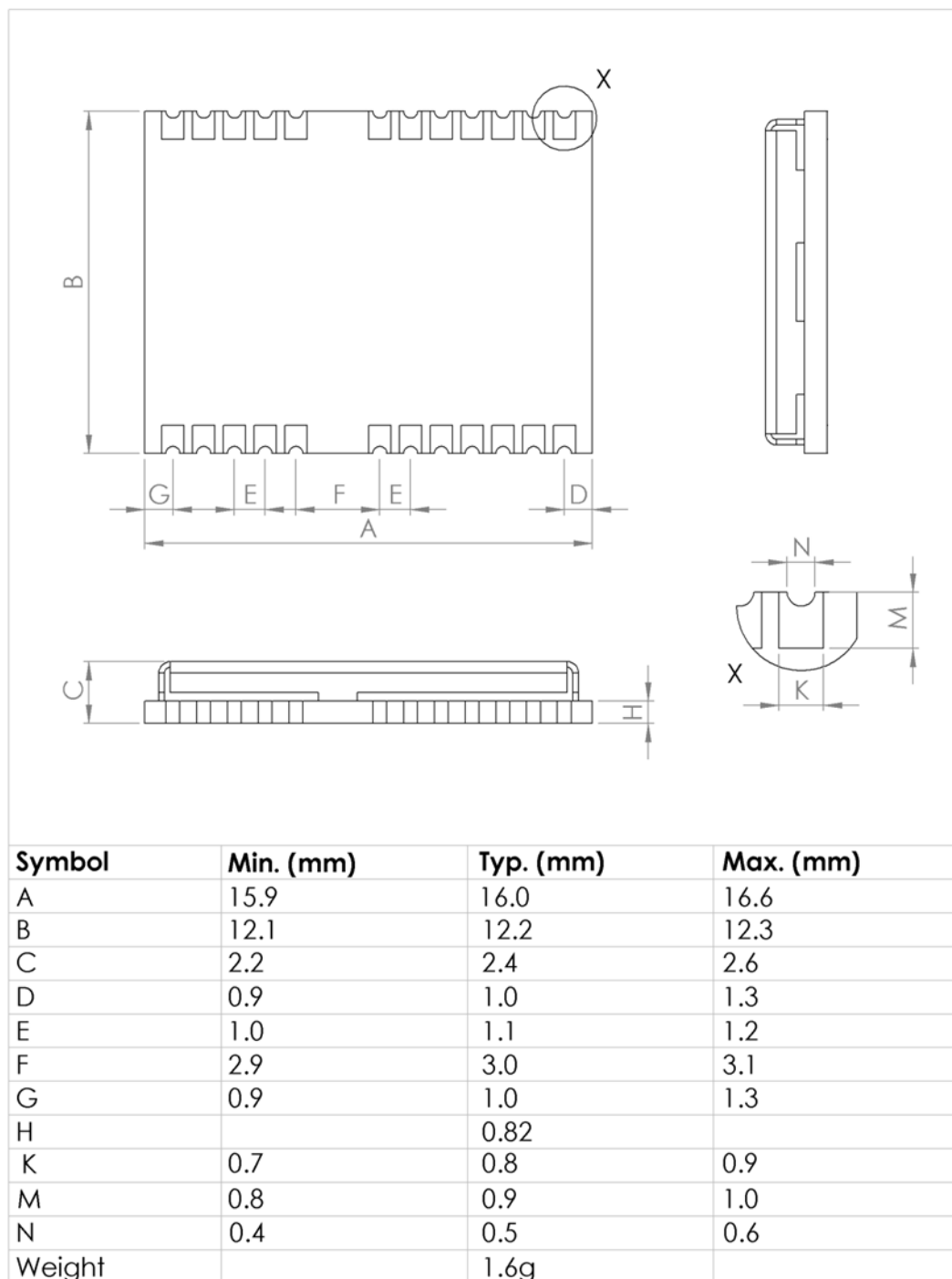
Figure 6: NEO dimensions
