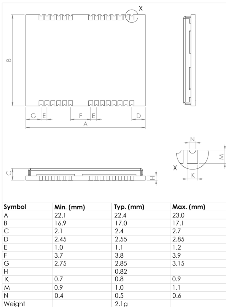
Figure 7: LEA dimensions
