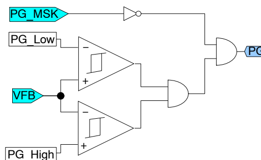
Figure 32. PG Block Diagram
