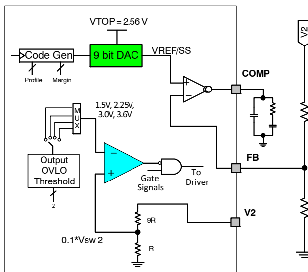
Figure 31. Output OVLO
