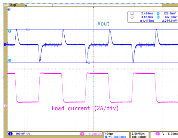
Figure 18. 20 V Load Step
