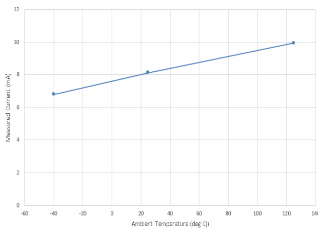
Figure 6. V1 Normal Current vs. Temperature
