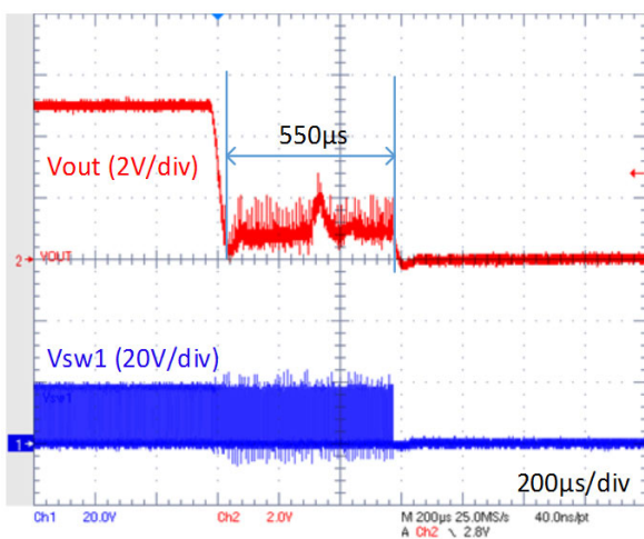
Figure 19. OCP Cycle-by-Cycle Waveform
