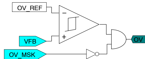
Figure 30. OV Block Diagram
