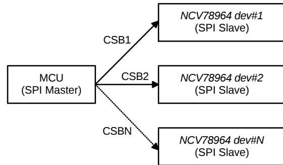
Figure 44. SPI Star Connection
