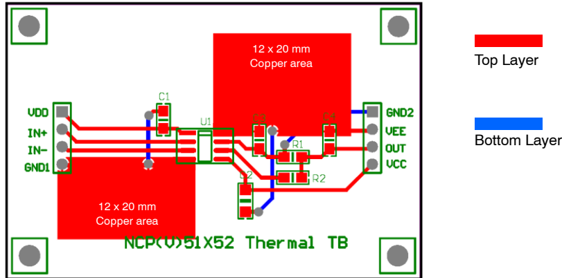
Figure 4. Reference Layout for the Type–A
