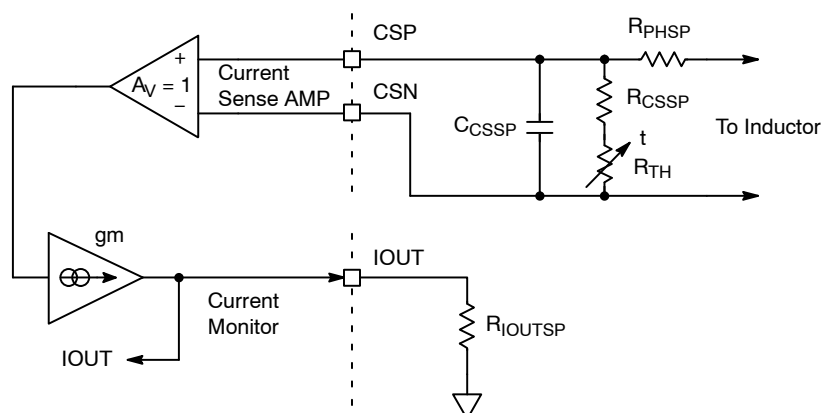
Figure 10. IOOUT Programming
