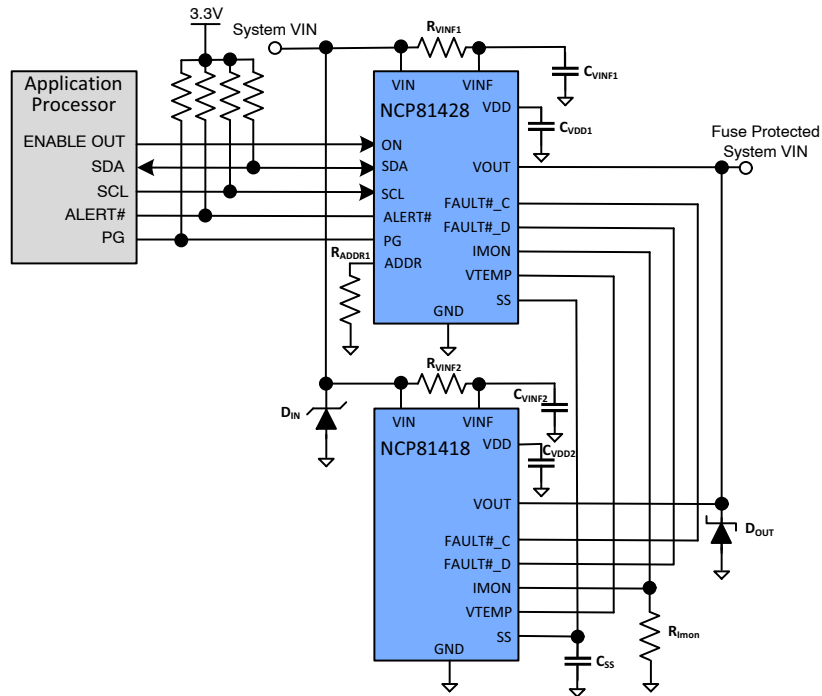
Figure 32. Application Circuit
