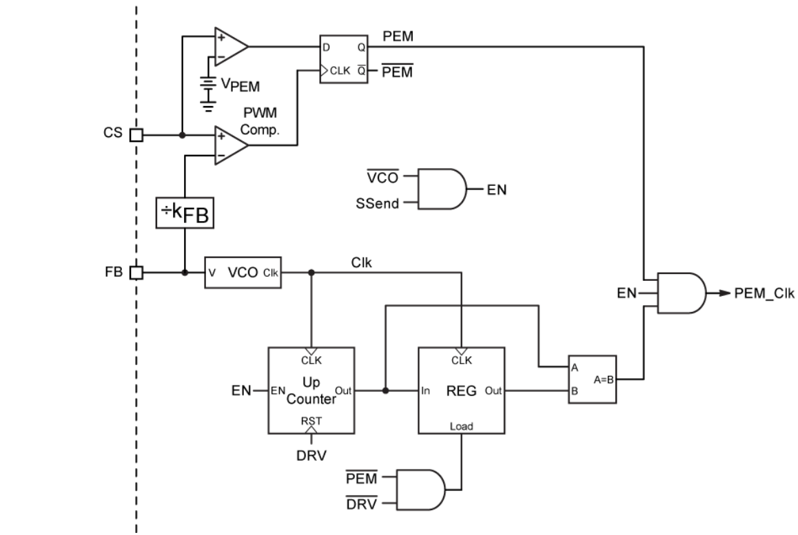
Figure 17. PEM Block Diagram
