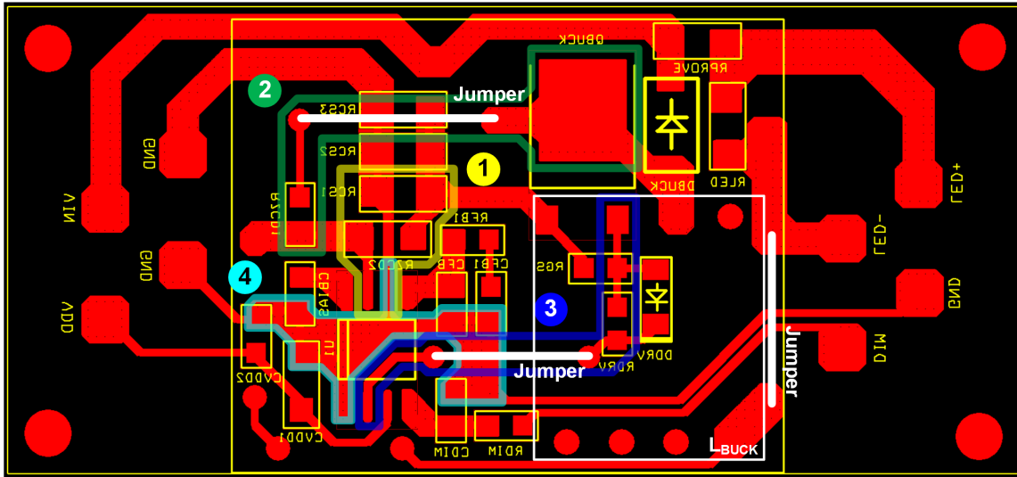
Figure 16. Layout Guidance
