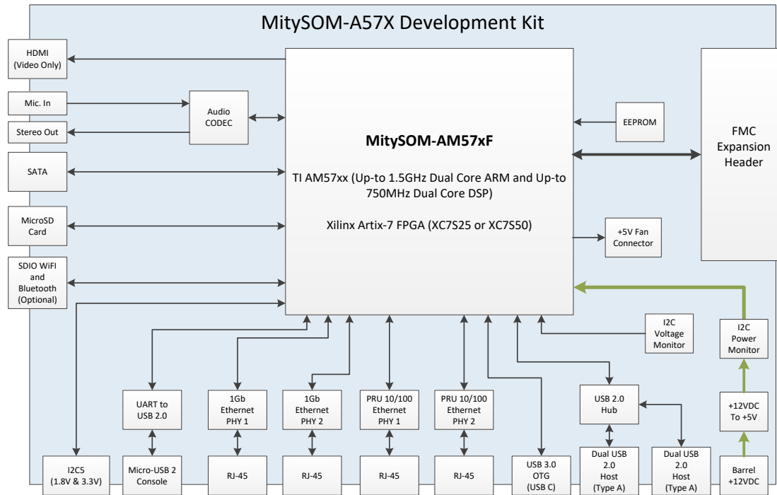
Figure 1: MitySOM-AM57x Development Kit Block Diagram
