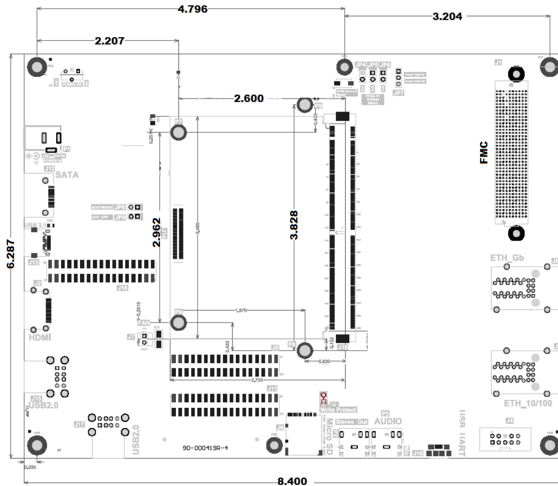
Figure 3: MitySOM-AM57x Development Kit Outline and Mounting Hole Locations (Top View, inches)
