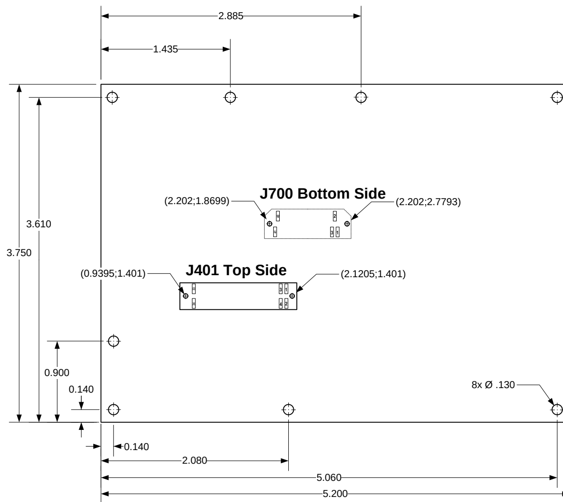
Figure 9: MitySOM-335x Development Kit Outline, Mounting Hole Locations, Hirose DF9-41P-1V(32) expansion header J700 and Molex 87832-3420 LCD header J401 (Top View, inches)
