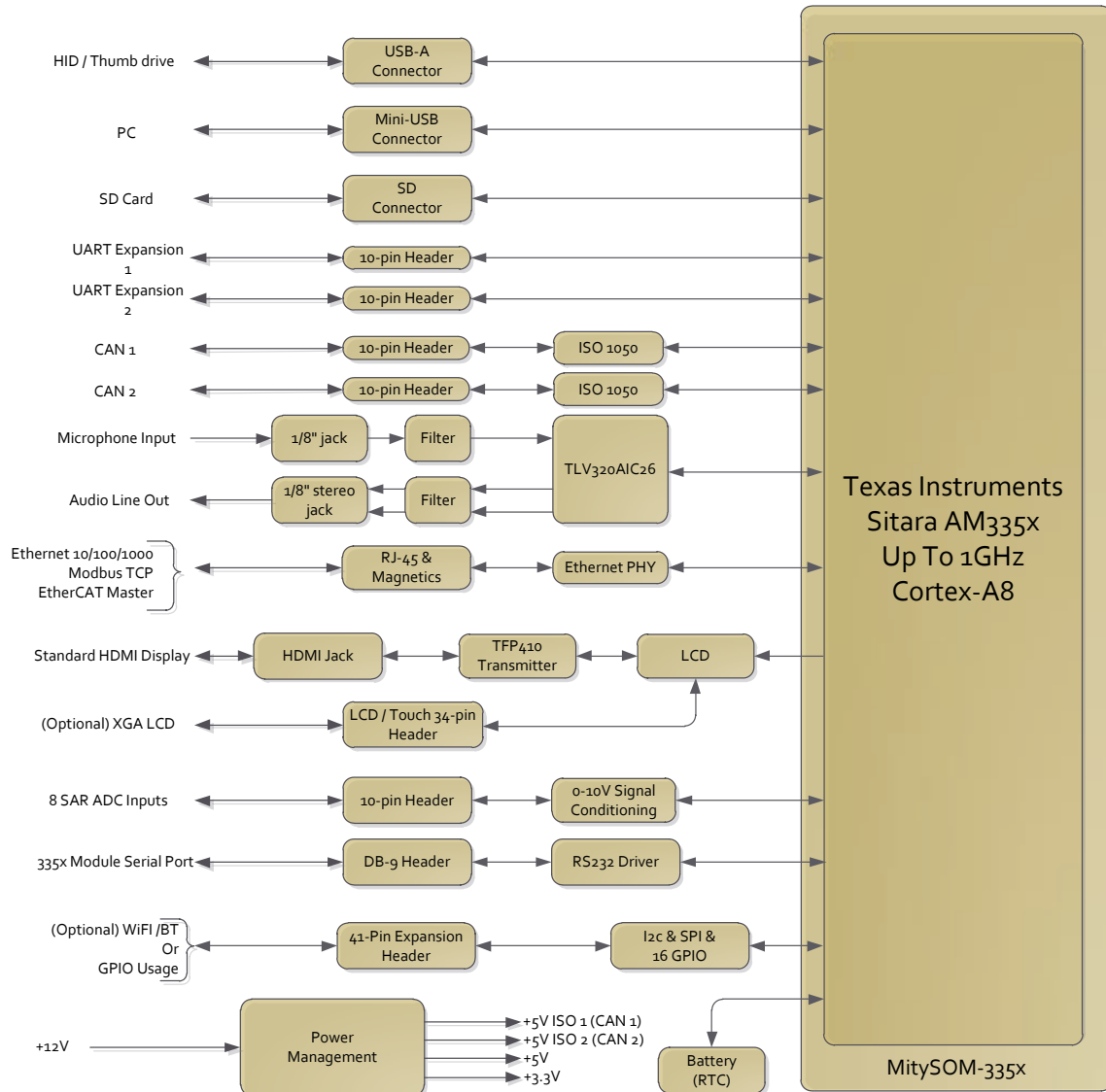
Figure 1: MitySOM-335x Development Kit Block Diagram
