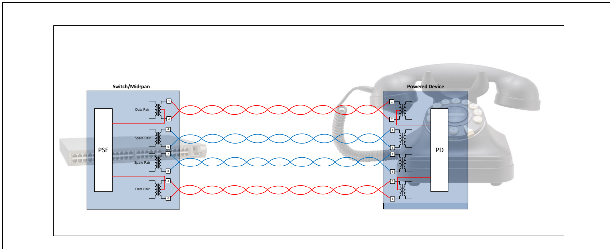
FIGURE 1: DATA DELIVERY OVER TWO PAIRS
