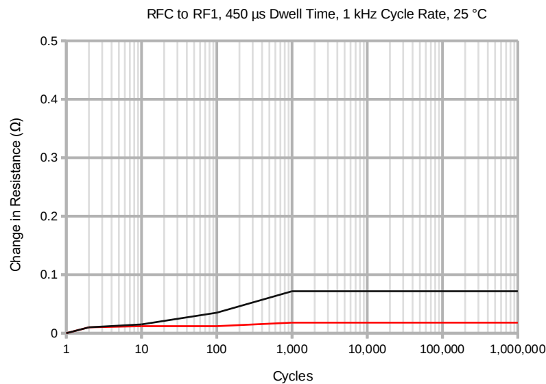
Figure 13. Typical R_{ON} Change Over Cycles and Current (450 \mu s Dwell Time)
