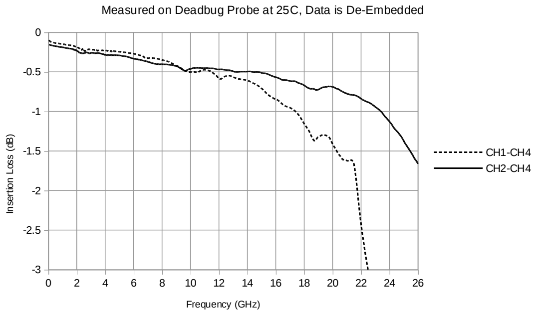
Figure 17. Super-Port Configuration Insertion Loss / S21
