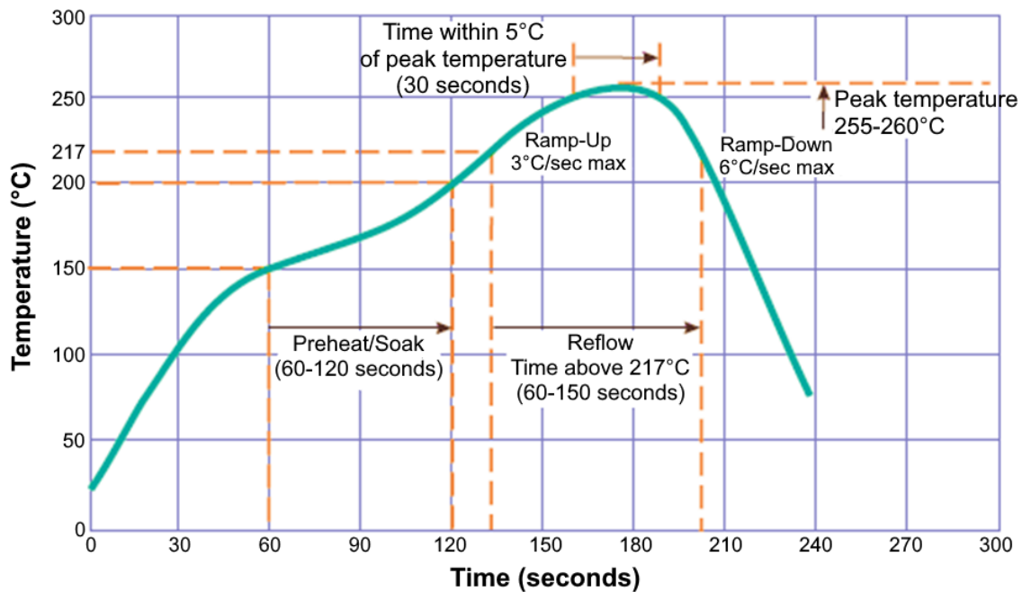
Figure 28. Reflow Profile
