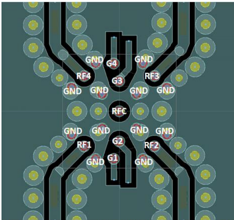
Figure 26. Super-Port Mode Layout Recommendation
