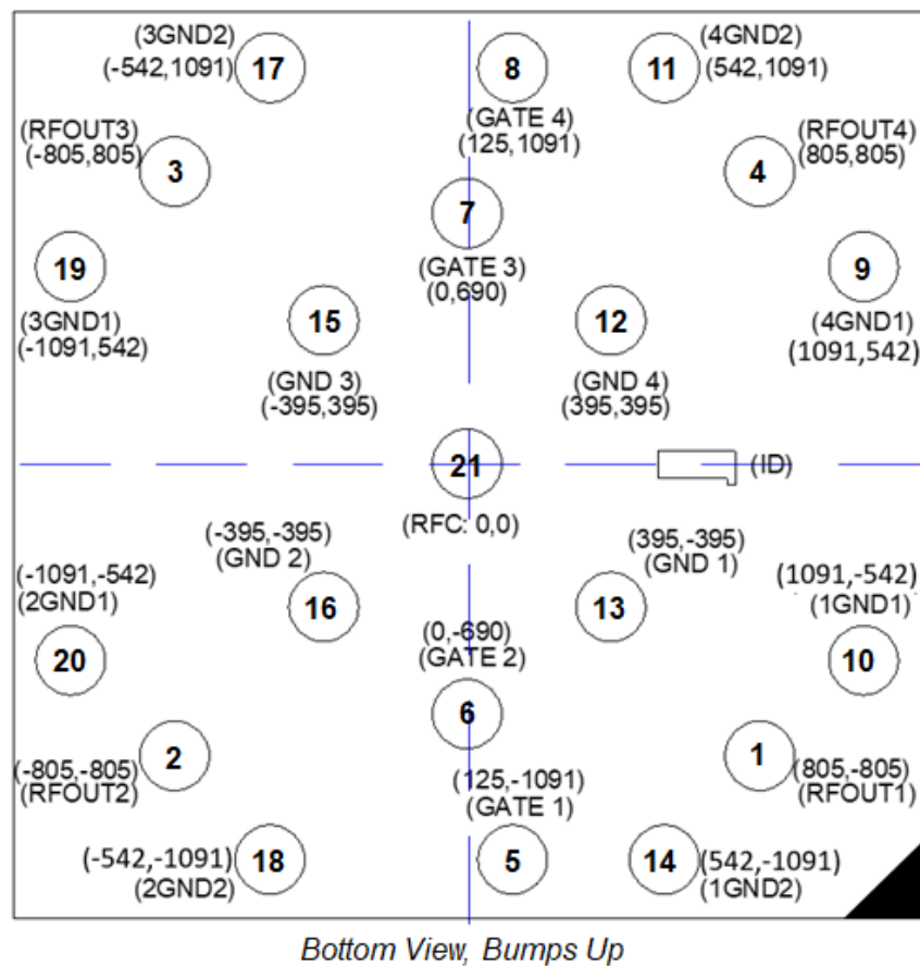
Figure 24. Bottom View/Bumps Up (0.0 at Die Center \mu\text{m} to Scale)
