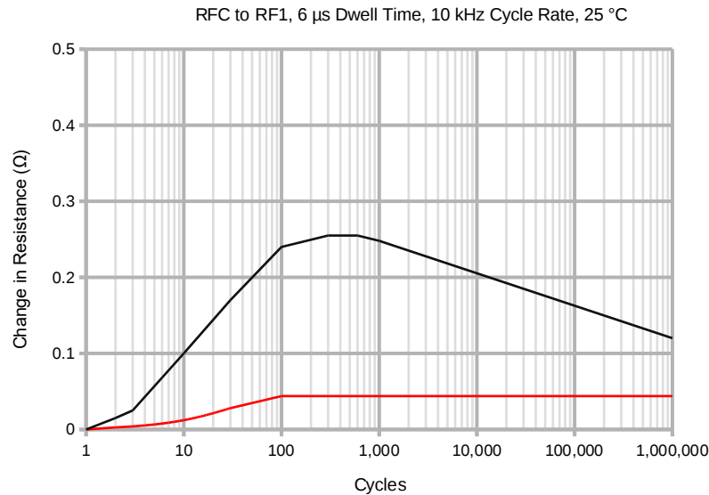
Figure 12. Typical R_{ON} Change Over Cycles and Current (6 \mu s Dwell Time)
