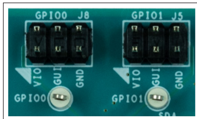
Figure 8. GPIO Headers
