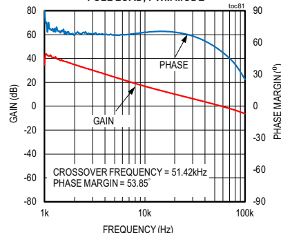
MAXM15462 BODE PLOT V_{IN} = 12V , ADJUSTABLE V_{OUT} = 1.5V , FULL LOAD, PWM MODE
