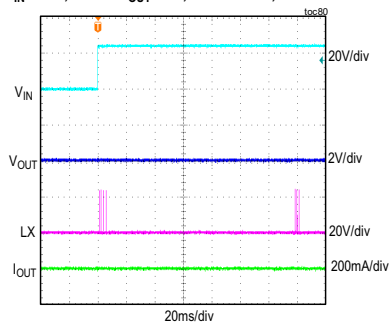
MAXM15464 OUTPUT SHORT DURING STARTUP V_{IN} = 24V , FIXED V_{OUT} = 5V , FULL LOAD, PWM MODE
