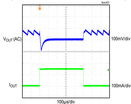
MAXM15064 LOAD TRANSIENT RESPONSE V_{IN} = 24V , ADJUSTABLE V_{OUT} = 3.3V , PFM MODE (LOAD CURRENT STEPPED FROM 5mA TO 150mA)
