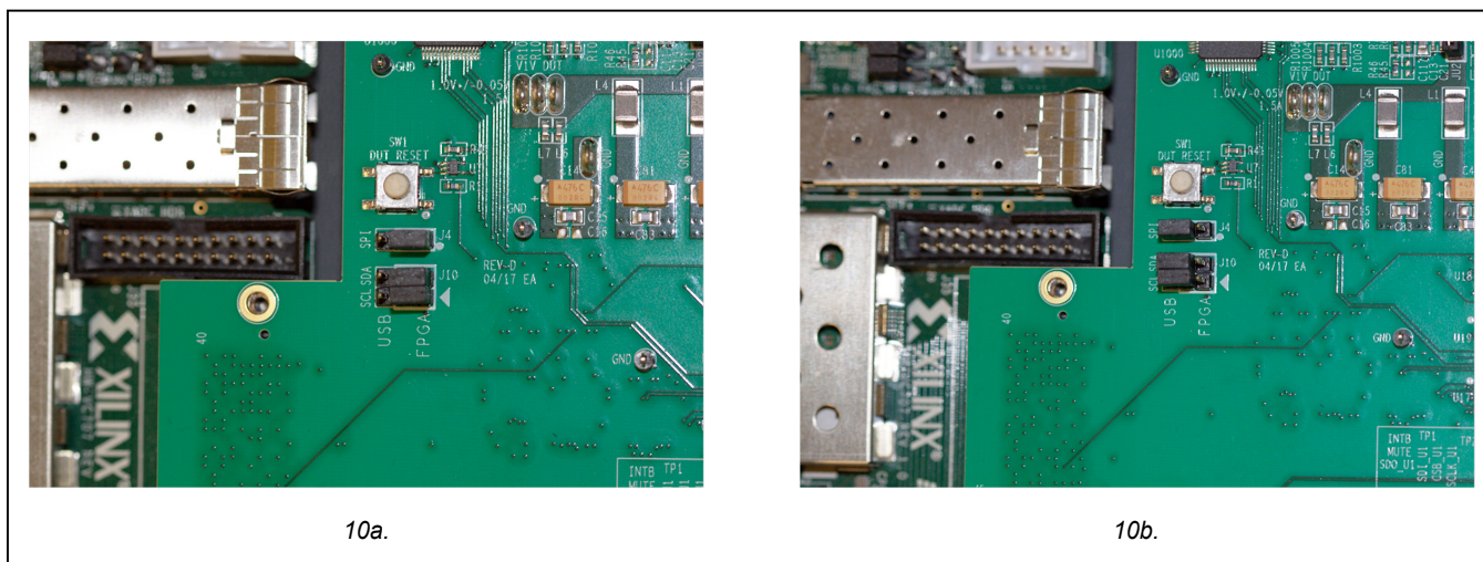
Figure 10. MAX5857 EV Kit Jumpers. 10a – default FPGA pass-through interface; 10b – on-board FTDI interface
