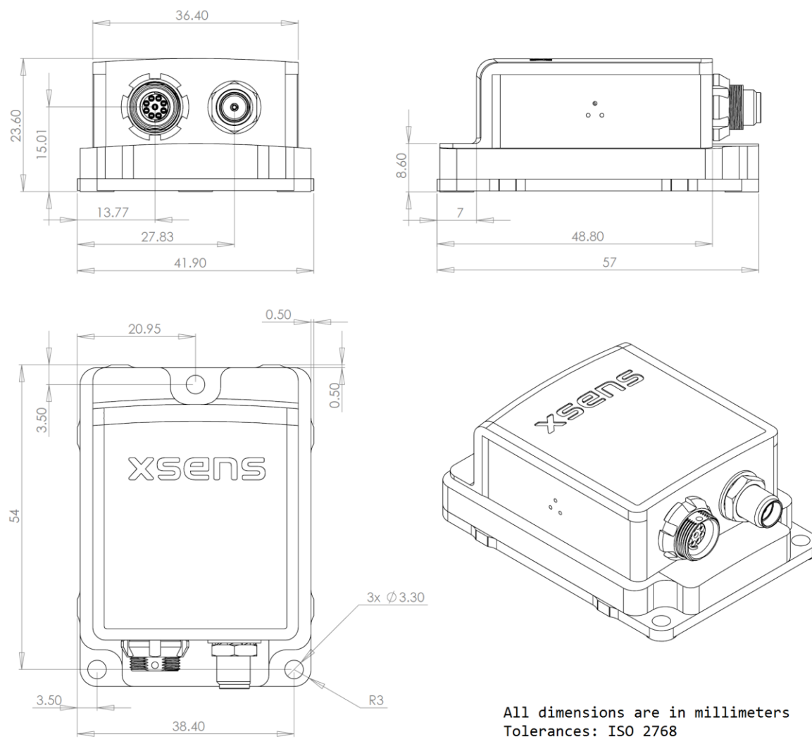
Figure 18: MTi-G-710 technical drawing
