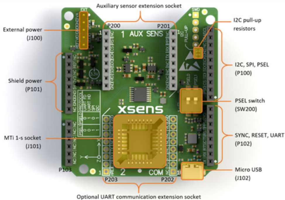
MTi 1-series Shield Board with connector designators
