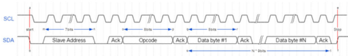
I 2 C write message operation
