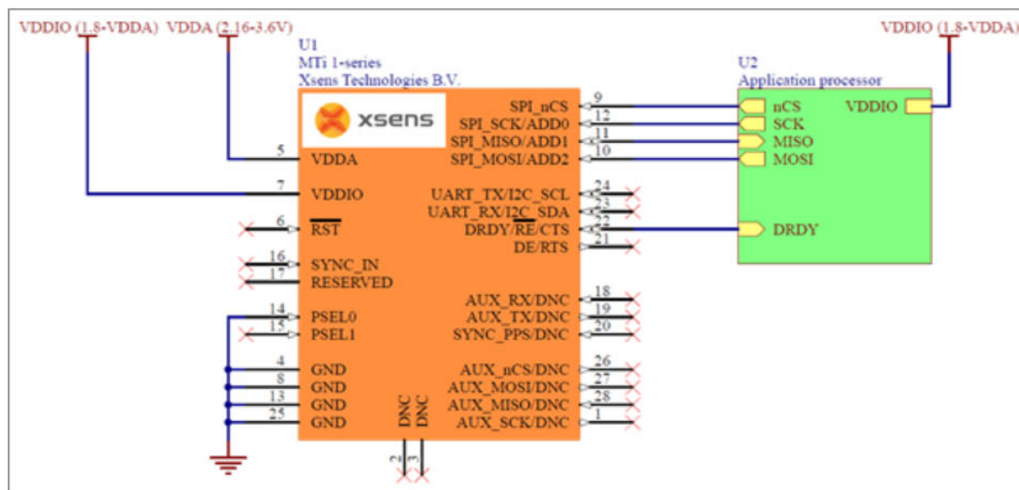
Connections (SPI interface)
