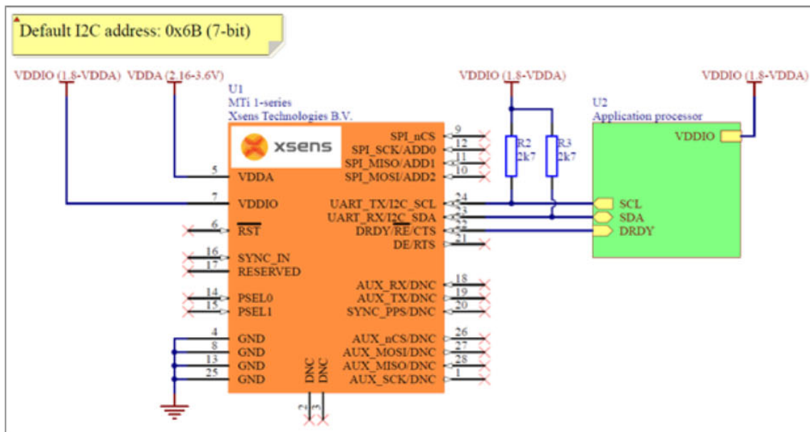
External components (I 2 C interface)
