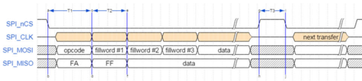
SPI timing
