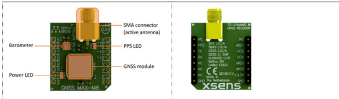
Top view (left) and the bottom view (right) of the MTi-7-DK GNSS daughter card
