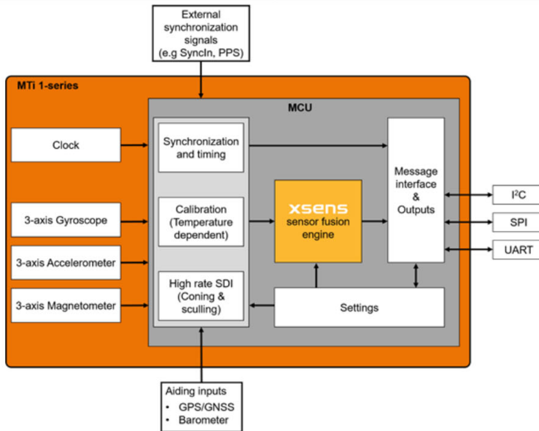
MTi 1-series module diagram
