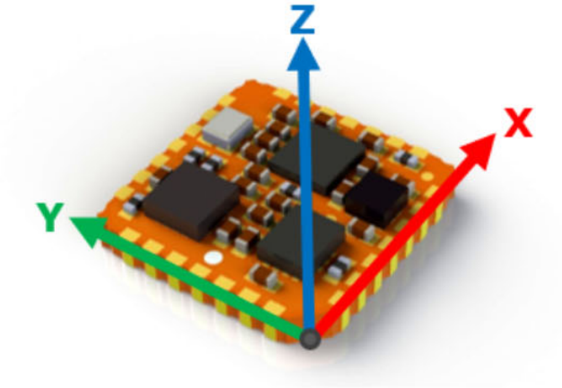
Default sensor fixed coordinate system for the MTi 1-series module
