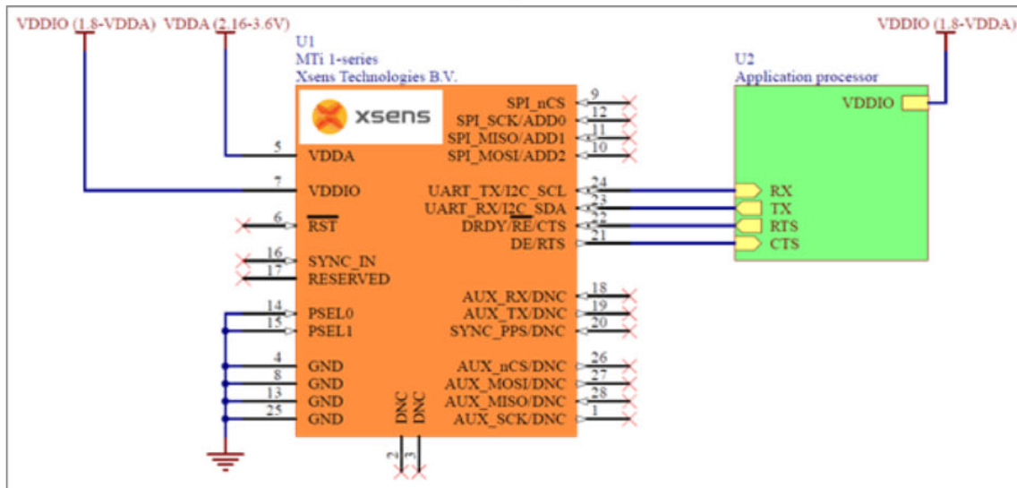
Connections (UART interface full-duplex)
