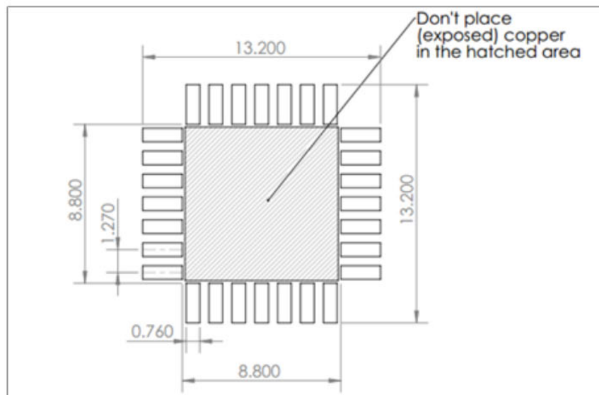
Recommended MTi 1-series module footprint
