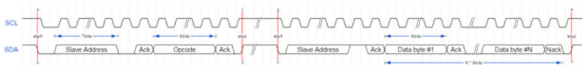
Read message operation with full write transfer and full read transfer (I 2 C)
