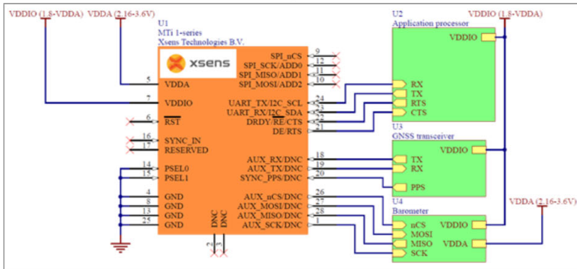
Connections (GNSS interface)
