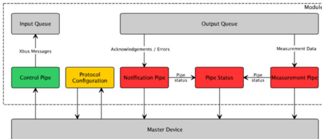
Data flows within MTSSP
