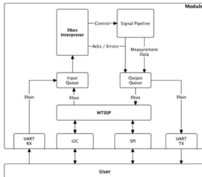
Communication architecture of MTi 1-series module (simplified)
