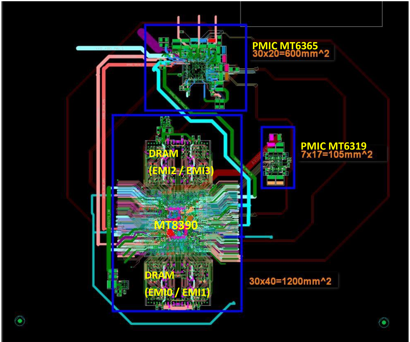
Figure 1-2. MMD Layout Dimension
