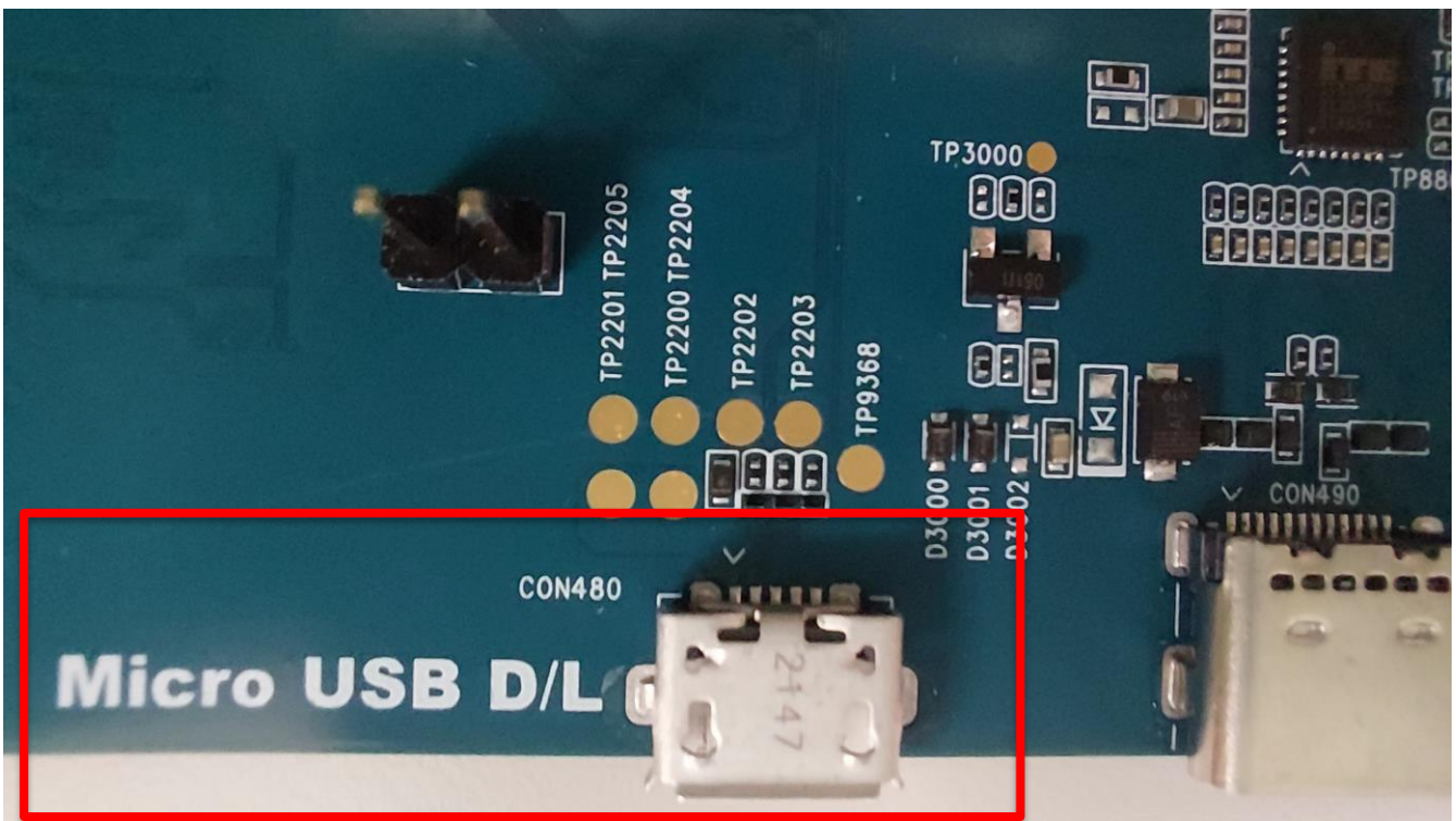
Figure 6-2.Download Port
