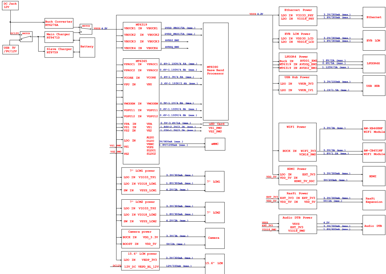
Figure 5-1. Power Distribution
