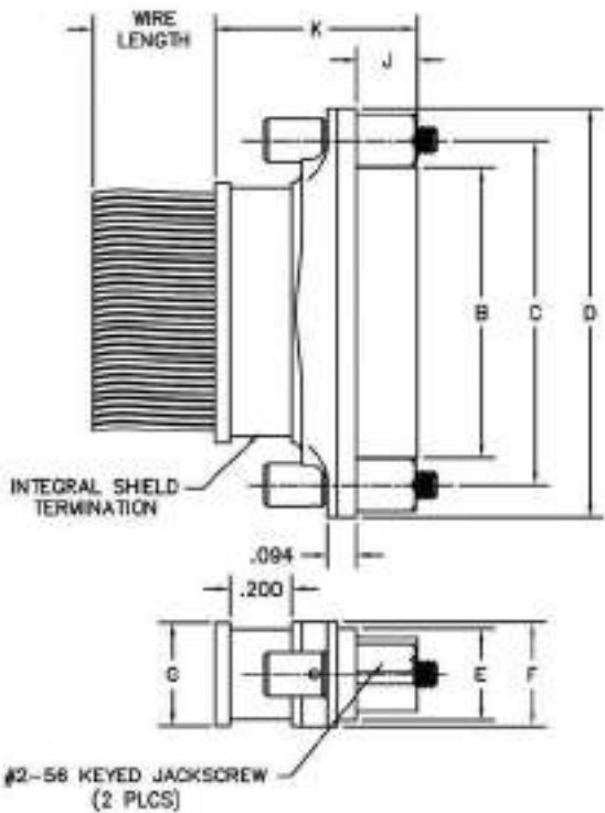
MM-2P2-031-101-44WA (PLUG)
