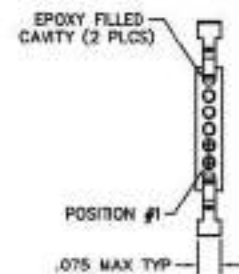
TERMINATION VIEW
