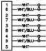
9 POSITION
