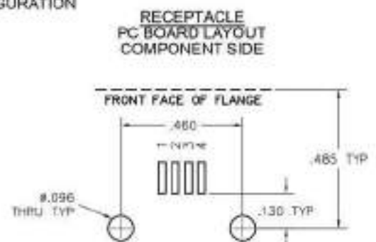
FOOTPRINT/PAD CONFIGURATION
