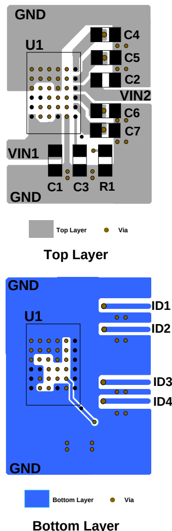
Figure 12: Recommended PCB Layout
