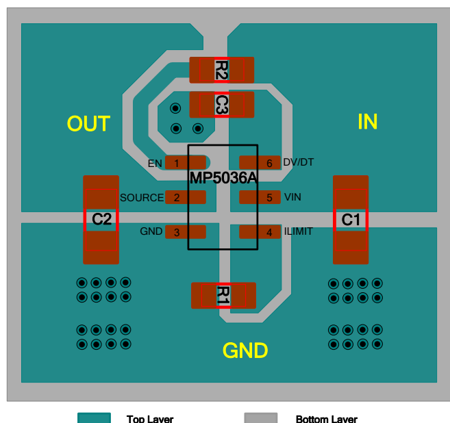
Figure 4: Recommended PCB Layout
