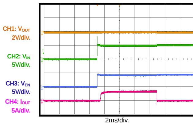
Short Circuit before Input Voltage Start-Up
