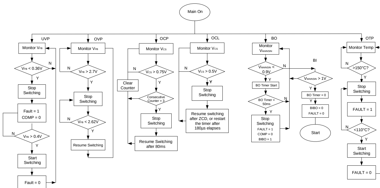
Figure 17: Control Flowchart
