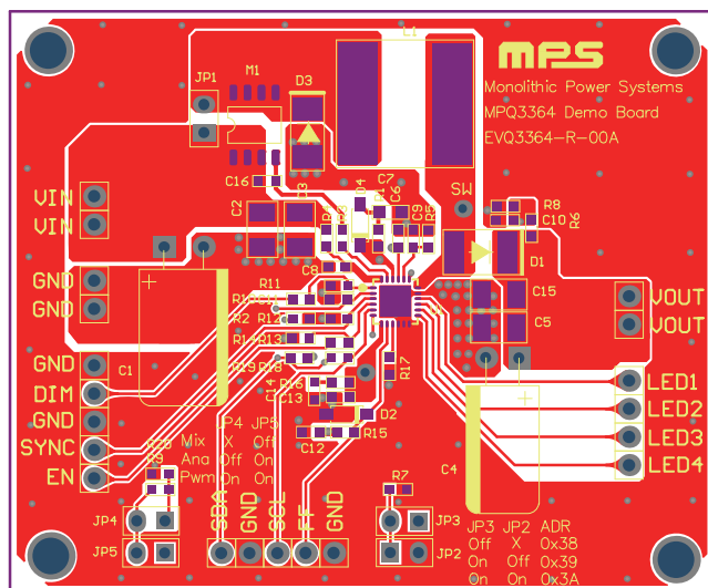
Figure 3: Top Layer
