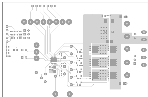
Figure 4: Top Layer
