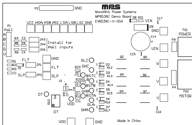
Figure 3: Top Silk
